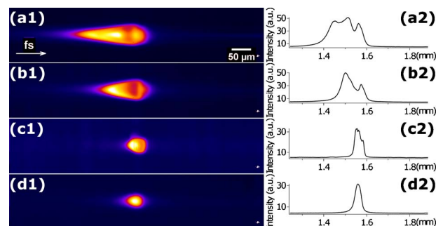
Fig. 2. (Color online) (a1),(b1),(c1) Plasma emission images obtained for pulses of energies of 9.6 \mu\text{J} and pulse durations of (a) 100, (b) 250, and (c) 550 fs. In (d), the pulse duration is 250 fs and the pulse energy is 4 \mu\text{J} . (a2),(b2),(c2),(d2) The corresponding intensity cross sections along the z -axis are shown in the right hand side of the image.
