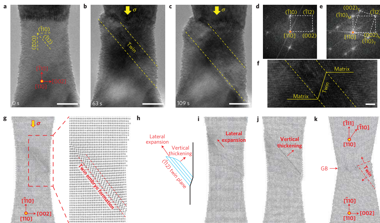
Figure 1 | Deformation twinning in a W bicrystal nanowire under [\bar{1}10] compression. a–c , Sequential TEM images showing deformation twinning in a W bicrystal nanowire (15 nm in diameter) at room temperature under a strain rate of 10^{-3} \text{ s}^{-1} , which is loaded along [\bar{1}10] and viewed along [110] . Scale bars, 5 nm. d,e , Fast Fourier transform pattern of the pristine W bicrystal and the deformation twin, respectively. f , Magnified TEM image showing the deformation twin. Scale bar, 1 nm. g , MD snapshot and zoomed-in image showing the nucleation of a deformation twin embryo in a W single-crystal nanowire. h , Schematic of the lateral expansion and vertical thickening of a twin band. i,j , MD snapshots showing the lateral expansion and vertical thickening of a deformation twin. k , Nucleation and thickening of a deformation twin in a W bicrystal nanowire. The crystal orientation is the same as that in Supplementary Fig. 2.
