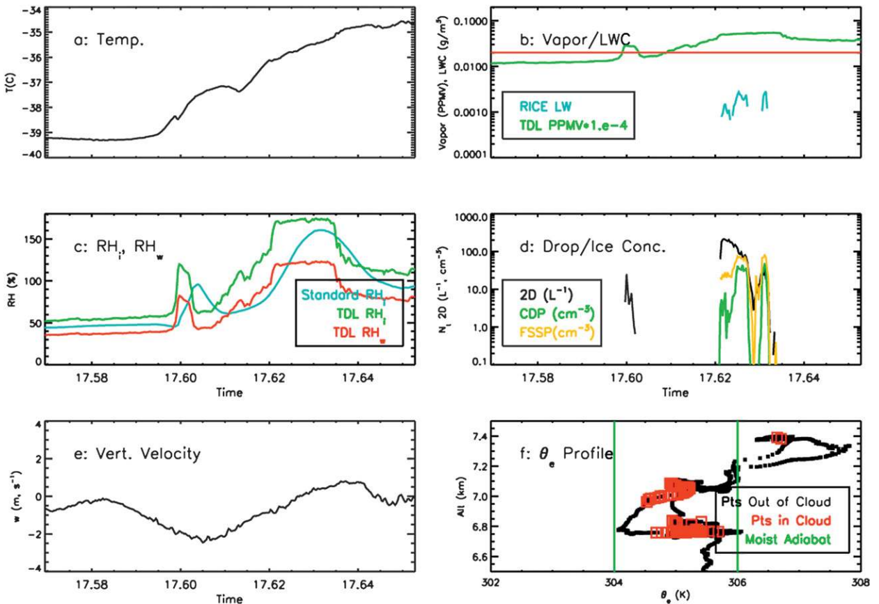
FIG. 5. Period 1 cloud properties: (a) temperature ( ^{\circ}\text{C} ); (b) water vapor content (ppmv) measured by the TDL hygrometer, and cloud LWC ( \text{g m}^{-3} ) measured by the Rosemount icing detector, with the red line denoting the LWC detection limit; (c) \text{RH}_i measured by standard and TDL hygrometers, as well as \text{RH}_w measured by the TDL hygrometer; (d) cloud particle (droplet-ice) concentrations measured by the following cloud particle probes: 2D ( \text{L}^{-1} ), CDP ( \text{cm}^{-3} ), and FSSP ( \text{cm}^{-3} ); (e) vertical velocity ( \text{m s}^{-1} ); and (f) \theta_e (K) with respect to altitude (km) for sampling in and out of cloud with the moist adiabat lines noted.
