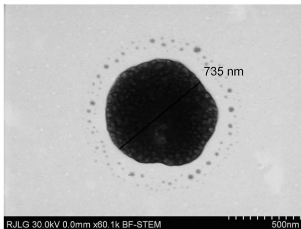
FIG. 1. STEM-EDX image of a 735-nm-diameter aged biomass-burning particle containing carbon, sulfur, oxygen, and potassium.
