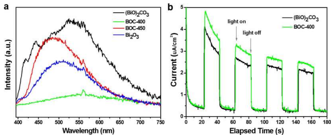
Figure 5. (a) Room-temperature PL spectra of the as-prepared samples. (b) Photocurrent plot of (BiO) 2 CO 3 and BOC-400 photoelectrodes.
