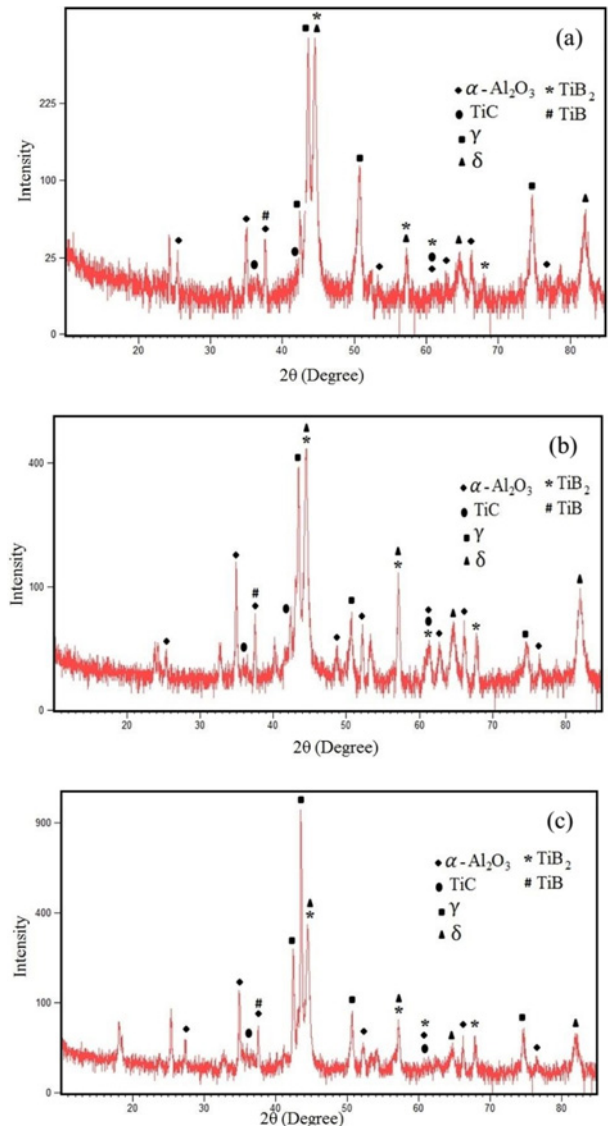
Fig. 8. The X-ray diffraction pattern of the samples: (a) T1, (b) T2, and (c) T3.
