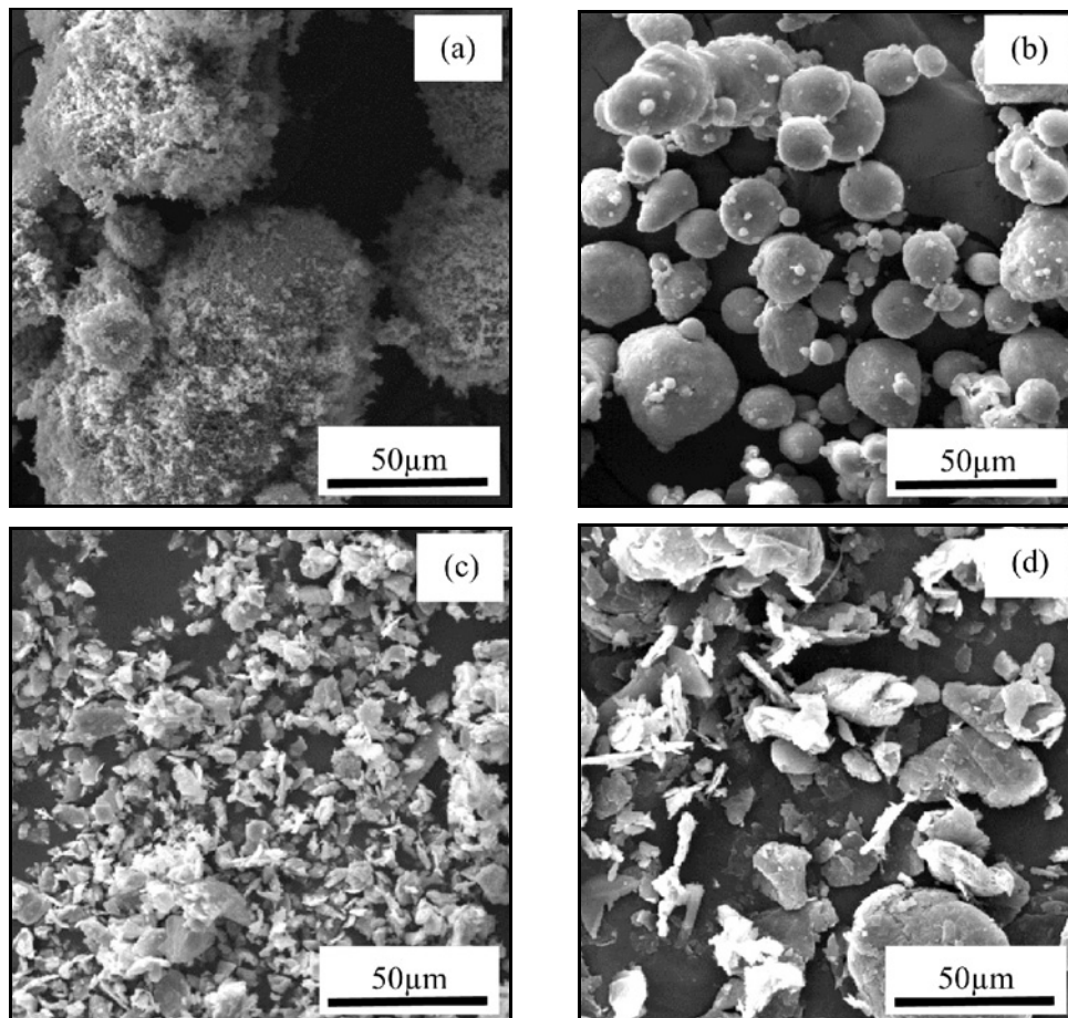
Fig. 1. SEM micrograph of powders: (a) TiO 2 , (b) Al, (c) B 4 C, and (d) C.
