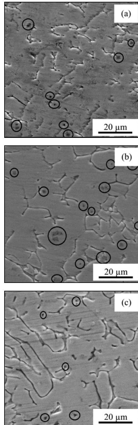
Fig. 5. SEM micrograph of coated layer of: (a) S1, (b) S2, (c) S3.
