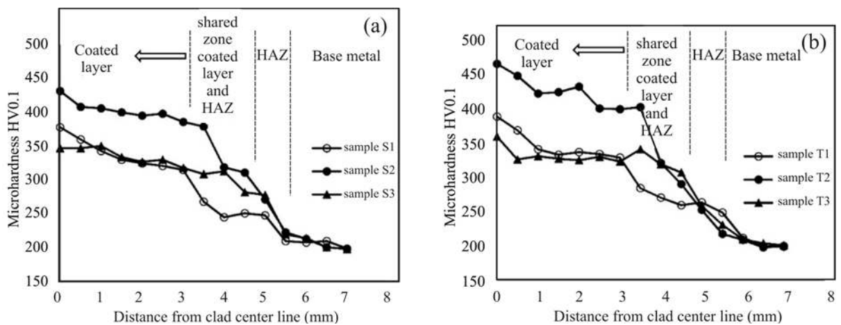
Fig. 12. The hardness distribution profile of (a) sample S1, S2, and S3 and (b) samples T1, T2, and T3.
