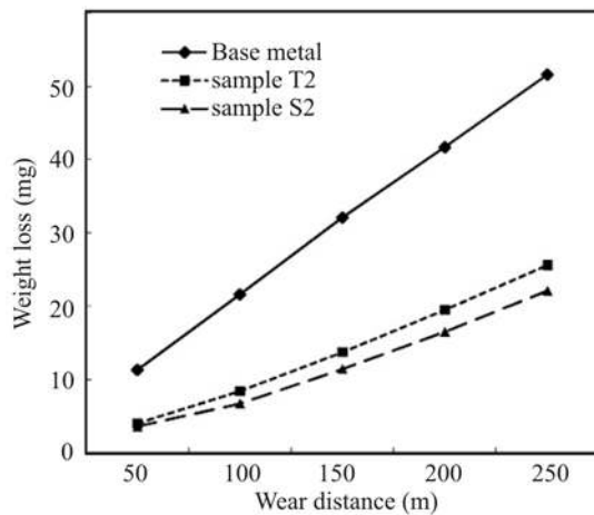
Fig. 13. Weight loss of base metal and samples S2 and T2.
