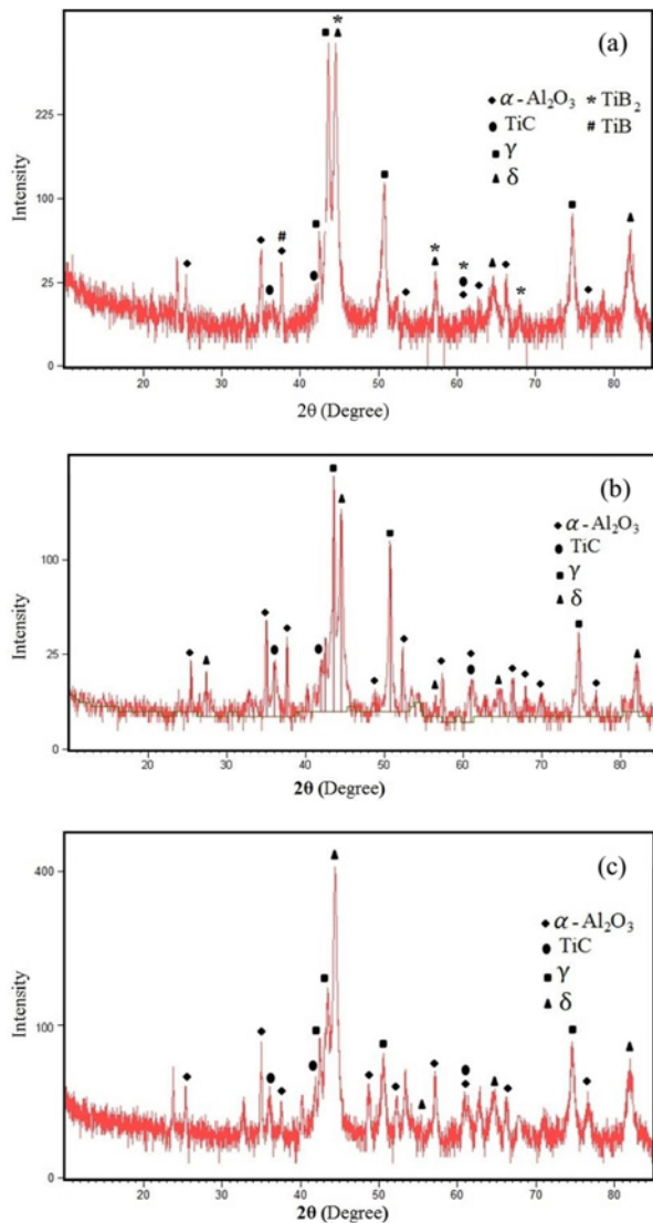
Fig. 4. X-ray diffraction pattern of the samples: (a) S1, (b) S2, (c) S3.
