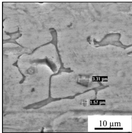
Fig. 6. TiC particle size in a matrix of sample S2.
