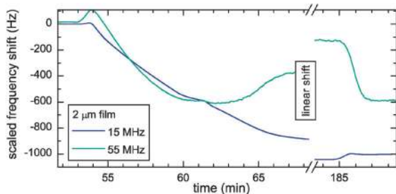
Fig. 4 Dye loading on 2 \mu\text{m} thick mesoporous \text{TiO}_2 films: Z907 exposure, 0.25 \text{ mM} in {}^t\text{BuOH} : \text{MeCN} (1 : 1) against a MeCN reference, showing different overtones at 15 or 55 \text{ MHz} .
