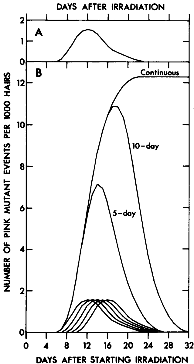
FIGURE 7. Daily changes of pink mutation frequency in the stamen hairs of KU 9 clone expected to occur after (A) a single acute exposure with 1 R and (B) a constant exposure at 1 R/day.
