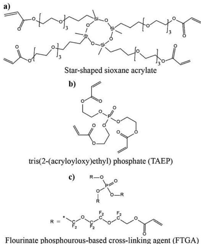
Fig. 20 (a) Chemical structure of the siloxane functionalized acrylate monomer; 437 (b) tris(2-(acryloyloxy) ethyl) phosphate; 438 and (c) the fluorinated phosphorous-based cross-linking agent. 439
