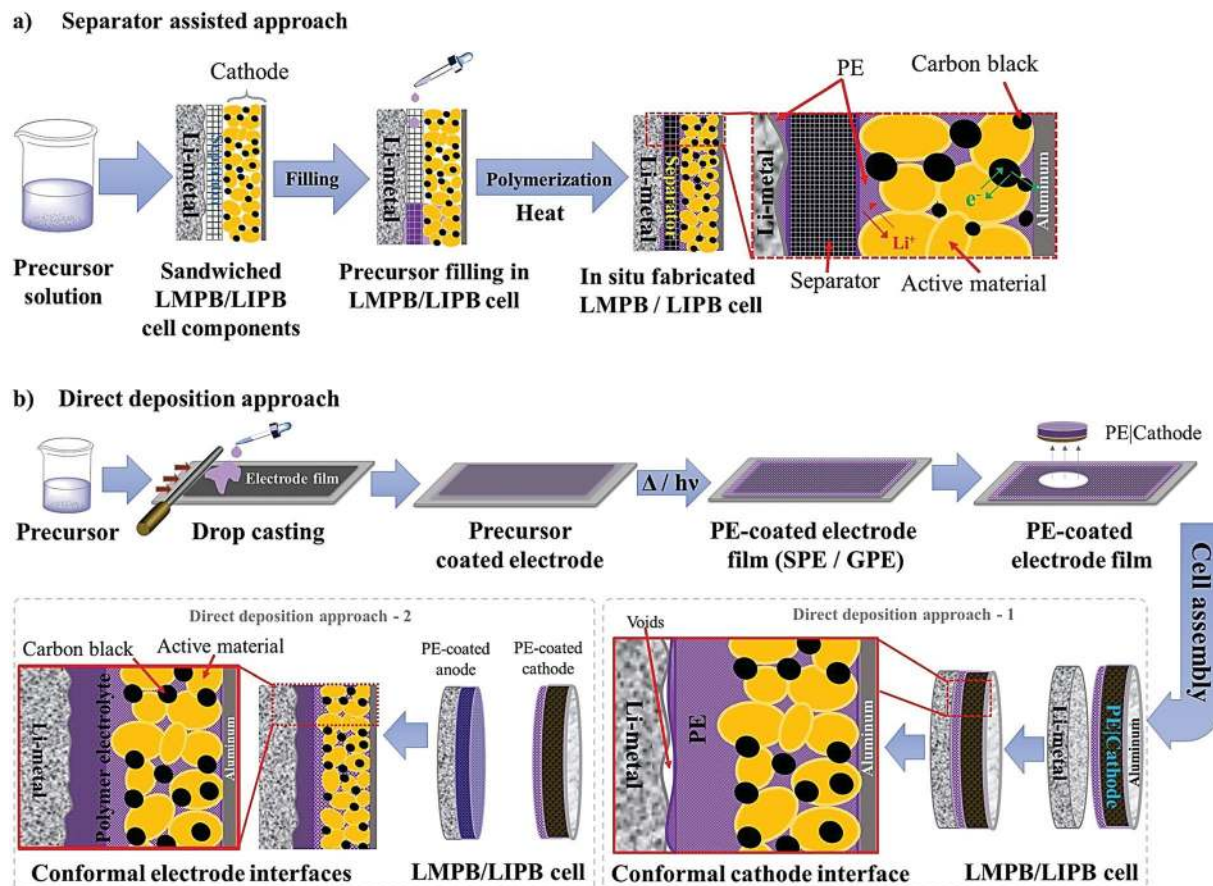
Fig. 8 (a) Separator assisted approach of the in situ processing of LMPB/LIPB cells. The precursor is filled and subjected to polymerization in a pre-assembled battery cell with the anode, cathode, and separator. Often, a precursor-soaked separator can also be used. (b) Direct deposition approach for the in situ processing of LMPB/LIPB cells, which involves the deposition of the precursor over the electrode film followed by free-radical or ionic polymerization methods, and subsequent cell fabrication. If the cathode alone is in situ processed (direct deposition approach 1), there is a chance that the electrode|electrolyte interface at the anode can be inferior. However, the inferior interface that may arise at one of the electrodes can be overcome by the in situ processing of both anode and cathode electrodes (direct deposition approach 2) followed by cell fabrication (for simplicity, only the in situ processing of LMPBs is illustrated, all the processes are applicable to LIPBs as well).
