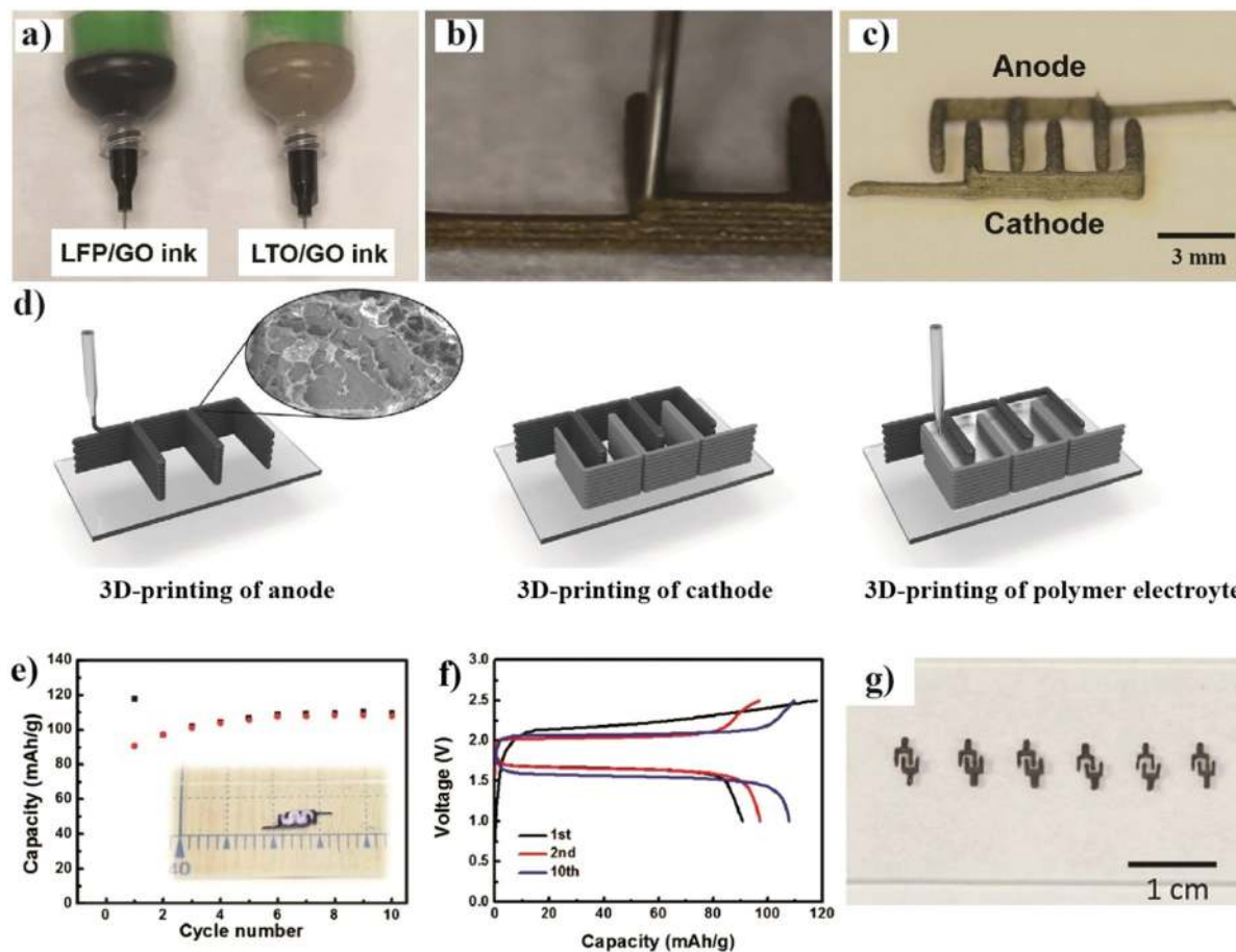
Fig. 53 (a) LTO/GO (anode) and LFP/GO (cathode) inks loaded in syringes used for the 3D-printing of mLEBs; patterning of the microelectrode (b) and the interdigitated electrode assembly (c); (d) step-wise 3D-printing of the anode, cathode, and the PE in the space between the anode and cathode fingers; (e) cycling stability and (f) galvanostatic charge–discharge profiles of the 3D-printed full cell as a function of the number of cycles; and (g) digital image of the 3D-printed interdigitated microelectrode arrays (reproduced/adapted from ref. 602 with permission from John Wiley and Sons, Copyright 2016 602 ).
