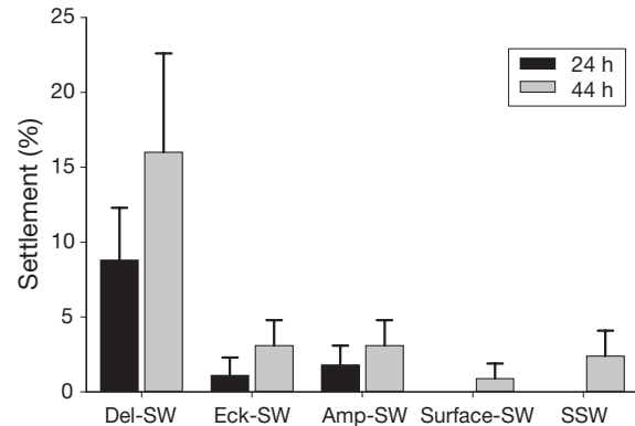
Fig. 3. Holopneustes purpurascens . Percent settlement (mean ± SE, n = 10, 10 larvae per dish) of aged larvae (3 wk post-fertilisation) after 24 and 44 h in response to seawater collected in situ near Delisea pulchra (Del-SW), Ecklonia radiata (Eck-SW) and Amphiroa anceps (Amp-SW), or at the sea surface (Surface-SW). Histamine (10 μM: not shown, 100% settlement at 24 h) and SSW were included as the positive and negative controls
