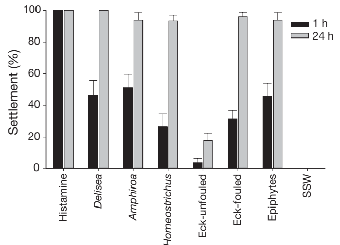
Fig. 2. Holopneustes purpurascens . Percent settlement of larvae (mean + SE, n = 10 , 5 larvae per dish) after 1 and 24 h in response to a range of host algae: Delisea pulchra , Amphiroa anceps , Homeostrictus olsenii , fouled Ecklonia radiata (Eck-fouled), unfouled E. radiata (Eck-unfouled) and the fouling epiphytes removed from laminae of E. radiata (epiphytes). Histamine (10 \mu\text{M} ) and SSW (sterile seawater) were included as the positive and negative controls
