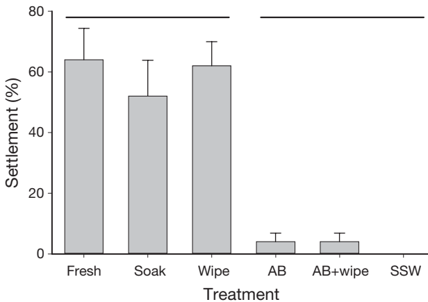
Fig. 4. Holopneustes purpurascens . Percent settlement of larvae (mean \pm SE, n = 10 , 5 larvae per dish) after 24 h in response to Amphiroa anceps that had been treated to reduce the surface bacterial community. The anti-bacterial treatment of A. anceps included 'AB' (streptomycin, penicillin G and kanamycin), 'wipe' (across agar) and 'AB + wipe' treatments. Control treatments were 'soak' (in SSW), 'fresh' A. anceps and SSW. Treatments that share a line induced a similar larval response (ANOVA, p < 0.001 ; Bonferroni pairwise comparisons, p < 0.001 )
