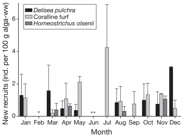
Fig. 1. Holopneustes purpurascens . Mean numbers (+SE) of new recruits (test diameter \leq 5 mm) found each month ( n = 2 yr) on Delisea pulchra , the coralline turf algae ( Amphiroa anceps and Corallina officinalis ) and Homeostrictus olsenii (total from n = 5 plants of each alga \text{mo}^{-1} standardised to number of recruits 100 \text{ g}^{-1} ww alga sampled). New recruits were not found on Ecklonia radiata or Sargassum vestitum at any time. *not sampled in Year 2, **not sampled in Years 1 and 2
