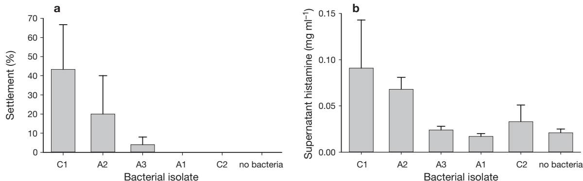
Fig. 5. Holopneustes purpurascens . (a) Percent settlement of larvae (mean \pm SE, n = 5 dishes, 5 larvae per dish) after 94 h in response to biofilms of bacterial isolates from the surface of Amphiroa anceps (A1, A2, A3) or Corallina officinalis (C1, C2; see Table 1). Biofilms containing no bacteria were used as the negative control and histamine (10 \mu\text{M} ) was used as the positive control (not shown). (b) Histamine concentration ( \mu\text{g ml}^{-1} \pm SE) of the supernatants from the culture of the bacterial isolates (n = 2)
