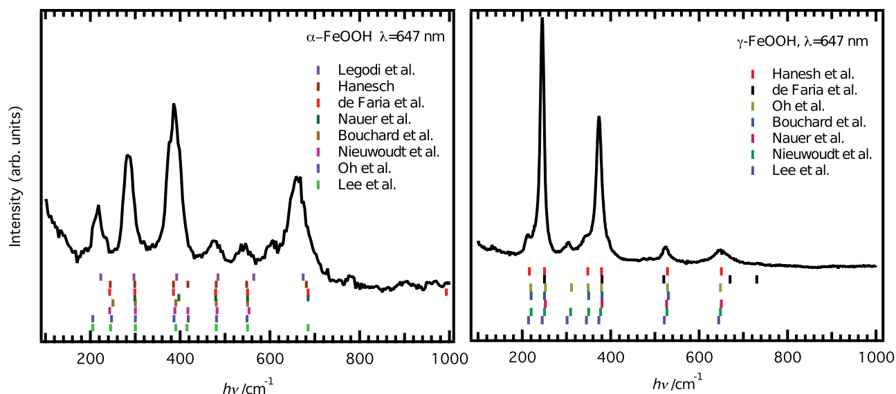
Figure 4. Ex situ Raman spectra of \alpha - and \gamma -FeOOH powder samples measured using 647 nm excitation wavelength. Raman-mode observed by other authors are indicated. 12,18,20–25
