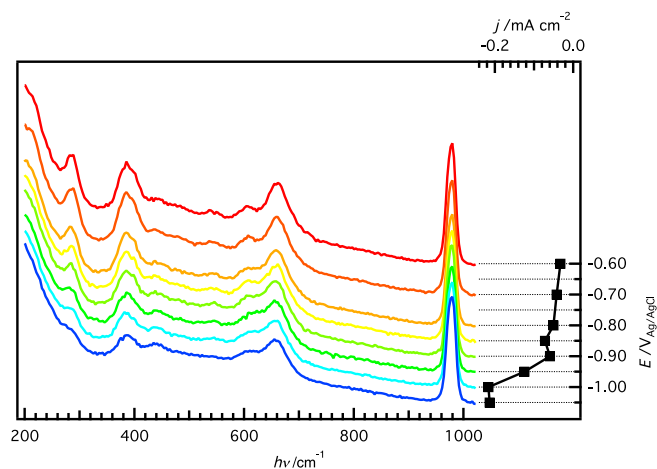
Figure 6. Evolution of Raman spectra with increasing cathodic load for \alpha -FeOOH using laser wavelength of 647 nm, together with steady-state currents for each potential. Each Raman spectrum is offset vertically to connect to the potential at which it was measured, as displayed on the right-hand scale.
