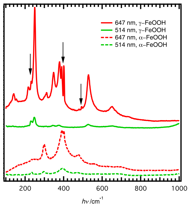
Figure 3. Ex situ Raman spectra of \alpha - and \gamma -FeOOH powder samples using red (647 nm) and green (514 nm) excitation laser lines. The spectra are offset vertically for clarity. In the measurement of \gamma -FeOOH using red laser line, some spurious spectral lines (confirmed to originate from illumination of the hallway outside the laboratory) appeared, indicated by arrows.
