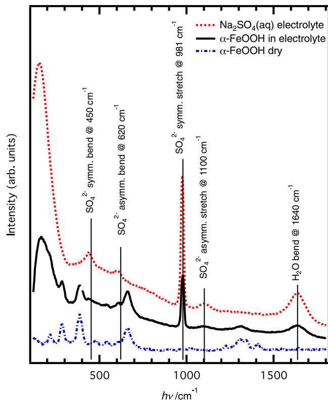
Figure 5. Raman spectra from \alpha -FeOOH sample inside the cell without electrolyte, spectra from the 0.2 M \text{Na}_2\text{SO}_4 electrolyte (set to pH 11 using NaOH) itself, and the sample measured in the electrolyte-filled cell. The known modes from water and sulfate ions are labeled. 26–28 The 647 nm laser line was used as excitation source. The three spectra have been offset vertically and rescaled to facilitate comparison.
