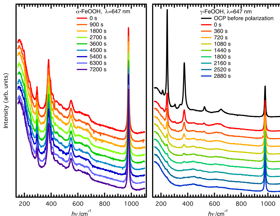
Figure 9. Evolution of Raman spectra with time during cathodic load of -950 mV vs Ag/AgCl for \alpha -FeOOH and \gamma -FeOOH using laser wavelength of 647 nm, as indicated. The labeled time points correspond to the time where the accumulation of Raman data commenced, with zero being start of polarization. In the right panel, the spectrum from the same sample before start of electrolysis is included for comparison.
