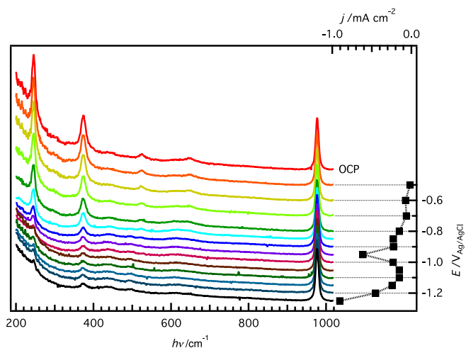
Figure 7. Evolution of Raman spectra with increasing cathodic load for \gamma -FeOOH using laser wavelength of 647 nm, together with steady-state currents for each potential. Each Raman spectrum is offset vertically to connect to the potential at which it was measured, as displayed on the right-hand scale.
