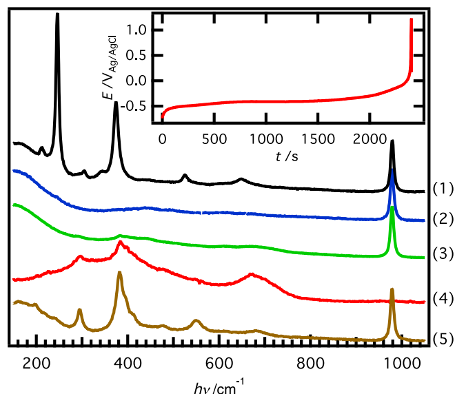
Figure 11. Reoxidation of \gamma -FeOOH on Ti substrate. First spectrum (1) is measured before cathodic load under OCP conditions. Spectrum (2) shows the sample toward the end to a cathodic polarization series. (Spectra (1) and (2) are identical to top and bottom spectra in the right panel of of Fig. 9) Spectrum (3) is measured from a sample that had been left in the electrolyte overnight after cathodic polarization followed by anodic re-oxidation (see inset). The sample was left in air several hours and measured again, spectrum (4). The bottom spectrum (5) is an in situ spectrum of \alpha -FeOOH without electrochemical polarization for comparison. The spectra are offset vertically for clarity, and rescaled to match the intensity of the sulfate peak at 981\text{ cm}^{-1} .
