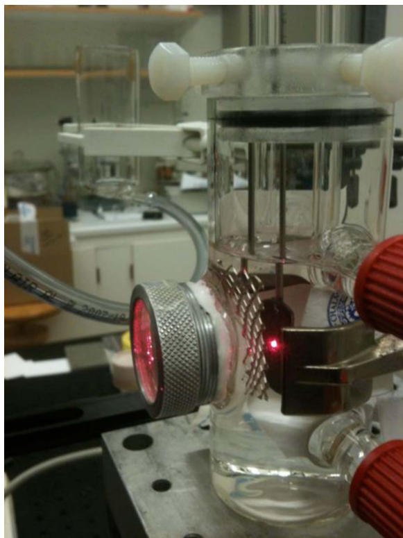
Figure 1. Photograph of the in situ Raman cell used in the study.
