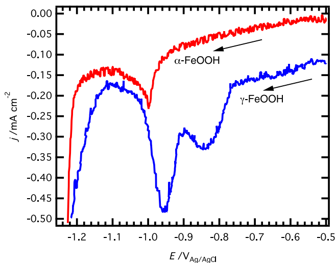
Figure 8. Slow potentiodynamic sweeps on both \alpha - and \gamma -FeOOH, clearly indicating the presence of a reduction peak at about -0.85 V vs. Ag/AgCl, unique for the \gamma -phase. Sweep rate was 0.1 \text{ mV}\cdot\text{s}^{-1} . Sweep direction indicated by arrows.
