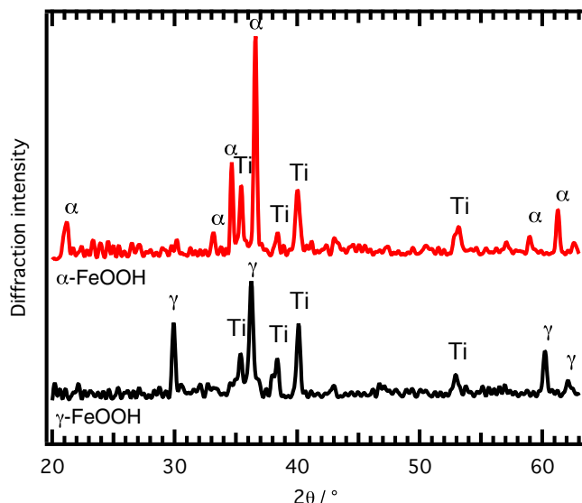
Figure 2. X-ray diffraction patterns, using \text{Cu K}\alpha radiation, of electrode samples. The position of peaks from \alpha - and \gamma -FeOOH as well as titanium metal, as known from databases are indicated. The curves are offset vertically for clarity.
