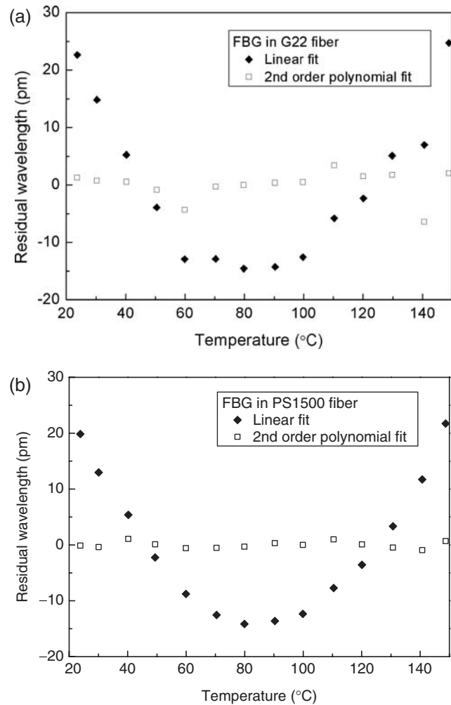
Figure 3. Residual wavelength shift for linear and second-order polynomial fit as a function of temperature change for both gratings written: (a) in the G22 and (b) in the PS1500 optical fibers.
