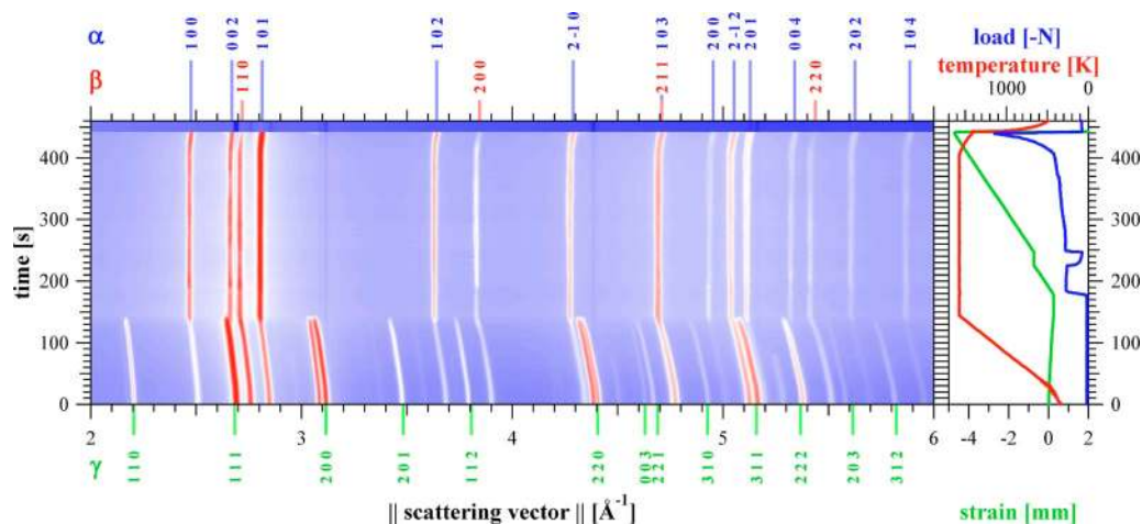
FIG. 2. (Color online) Color coded powder diffraction patterns obtained by azimuthal integration of the time frames in Fig. 1 vs scattering vector q=4\pi/\lambda \sin(2\theta/2) on the abscissa evolving in time on the ordinate to the left. Because of the tetragonality of \gamma -TiAl ( L1_0 structure), some reflections appear as double lines. For simplification, however, indices are given for a fcc lattice. The deformation parameters (compressive mode) are given to the right.
