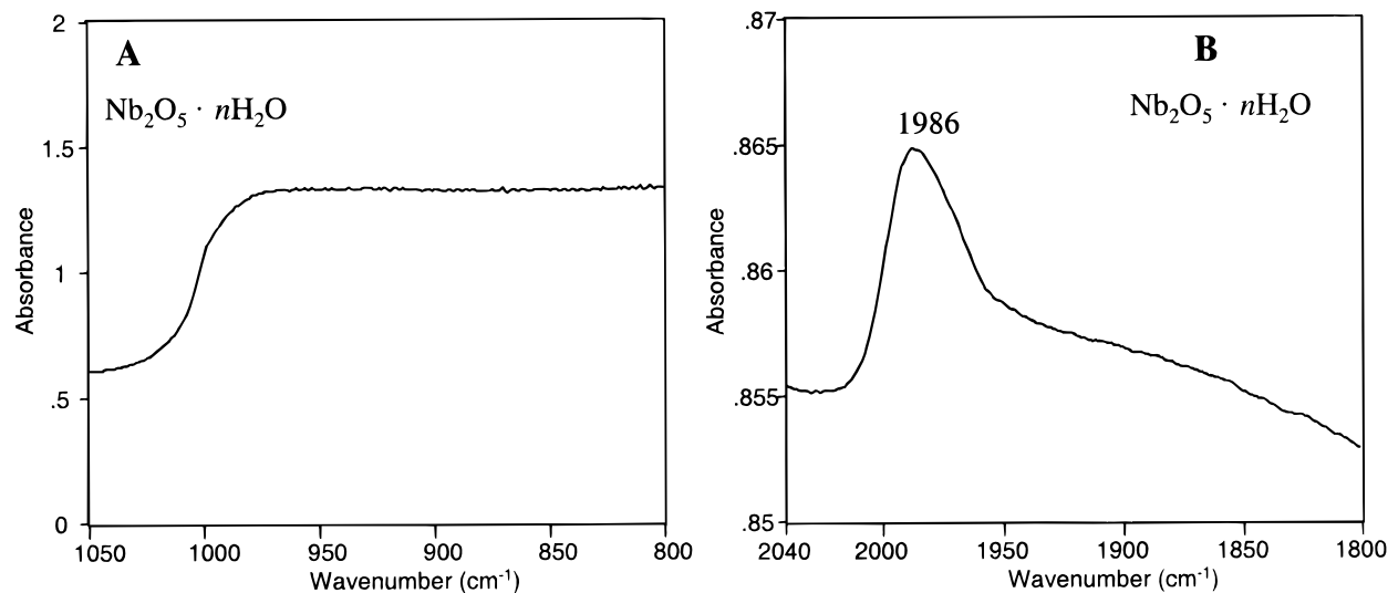
Figure 1. Fundamental (A) and overtone (B) IR spectra of \text{Nb}_2\text{O}_5 \cdot n\text{H}_2\text{O} . The ordinate scale has been expanded in the overtone spectrum for clarity.
