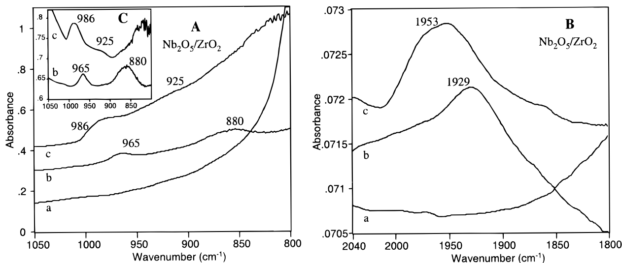
Figure 3. Fundamental (A) and overtone (B) IR spectra of \text{Nb}_2\text{O}_5/\text{ZrO}_2 . The ordinate scale has been expanded in the overtone spectra for clarity. The inset (C) shows the baseline-subtracted spectra in the fundamental region. Spectra are labeled as follows: a = \text{ZrO}_2 support; b = 1 wt % \text{Nb}_2\text{O}_5/\text{ZrO}_2 ; c = 5 wt % \text{Nb}_2\text{O}_5/\text{ZrO}_2 .
