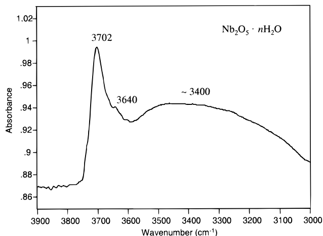
Figure 6. IR spectrum of the hydroxyl region of \text{Nb}_2\text{O}_5 \cdot n\text{H}_2\text{O} .
