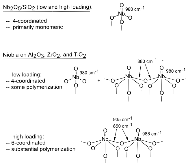
Figure 7. Schematic drawing of the molecular structures present on supported niobia catalysts under dehydrated conditions. Assignments of the Nb—O—Nb modes, by analogy to assignments in supported chromia systems, 35 include assignment of the vibrational band at \sim 880 – 935\text{ cm}^{-1} to \nu_s([-\text{O}-\text{Nb}-\text{O}-]_n) , while the band at \sim 650\text{ cm}^{-1} is assigned to \nu_s(\text{Nb}-\text{O}-\text{Nb}) .
