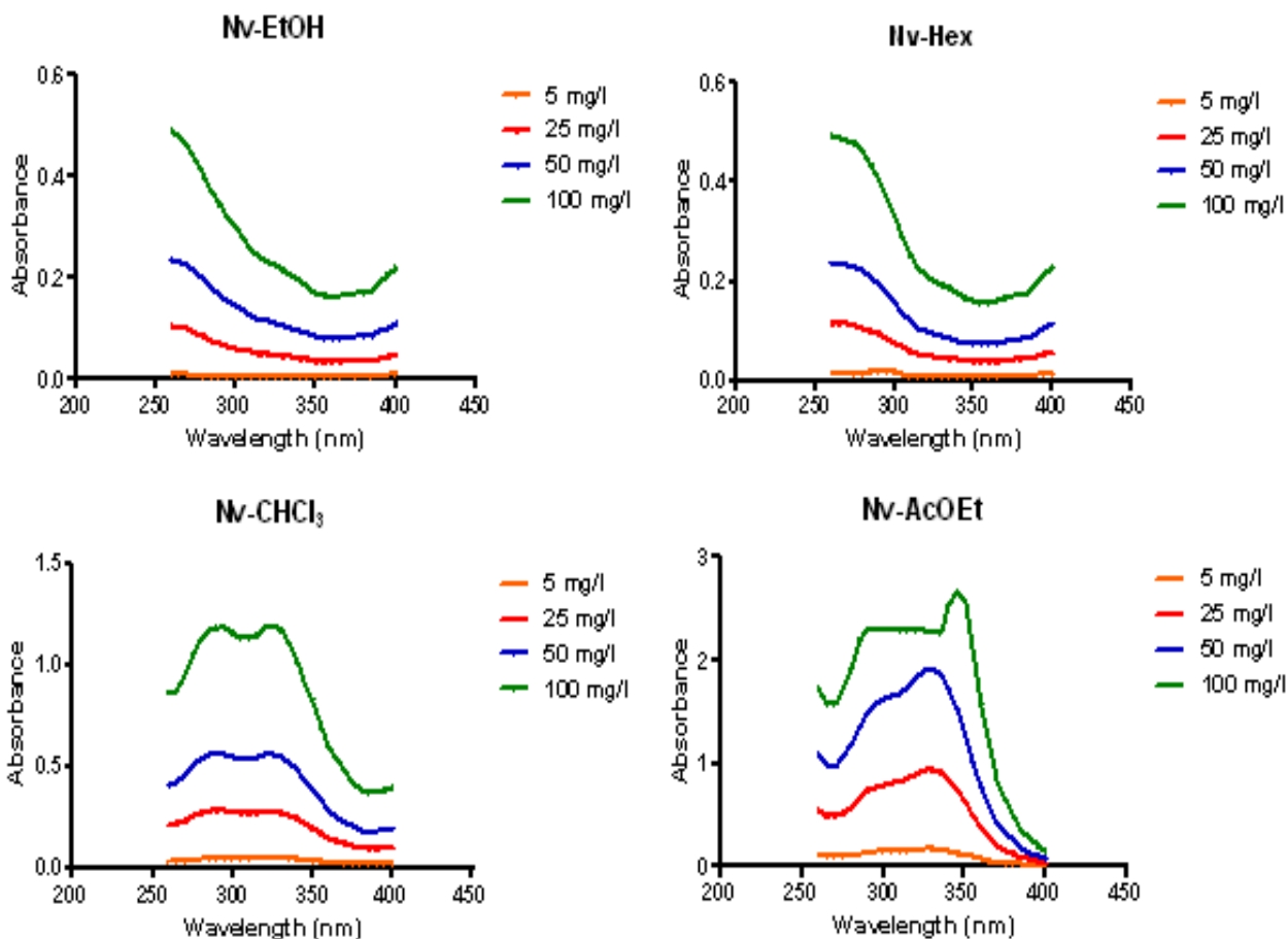
Fig. 1: Spectrophotometric absorption profile of dried extracts of Neoglaziovia variegata (260-400 nm).
