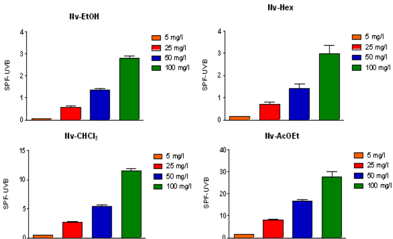
Fig. 2: Sun Protection Factor (SPF) in vitro of the dried extracts of Neoglaziovia variegata .
