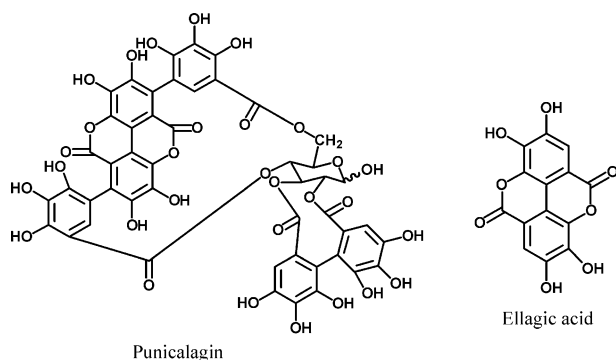
Fig. 1. Structures of punicalagin, the major polyphenol antioxidant ingredient in PJ, and EA.
