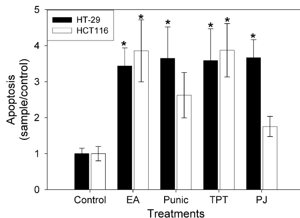
Fig. 5. Effects of punicalagin, EA, TPT and PJ on apoptosis in human colon HT29 and HCT116 cells. Cells were treated with samples at 100 µg/ml for 24 h before they were harvested for analyses using the Cell Death Detection ELISA PLUS Assay. Values are mean±S.D., n=3 . Asterisk indicates a significant difference compared to P \leq 0.01 , two-tailed t test.
