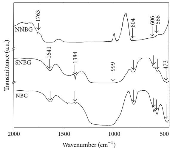
FIGURE 2: FTIR spectra of bioactive glass nanocomposites.
