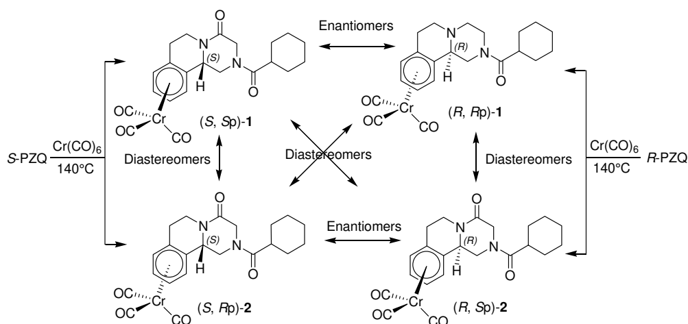
Scheme 2. Synthesis of 3 and optically pure (\eta^6\text{-PZQ})\text{Cr}(\text{CO})_3 derivatives. Note that Praziquanamine, 3 and Iso- 3 are racemates.
