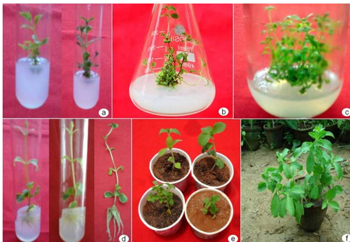
Figure 1. The successive stages of in vitro propagation of Stevia rebaudiana . (a) Direct regeneration of shoot from explant, (b) Initiation of multiple shoot formation, (c) Development of more number of multiple shoot, (d) Root formation from regenerated shoot (e & f) Hardening and establishment regenerated plants.
