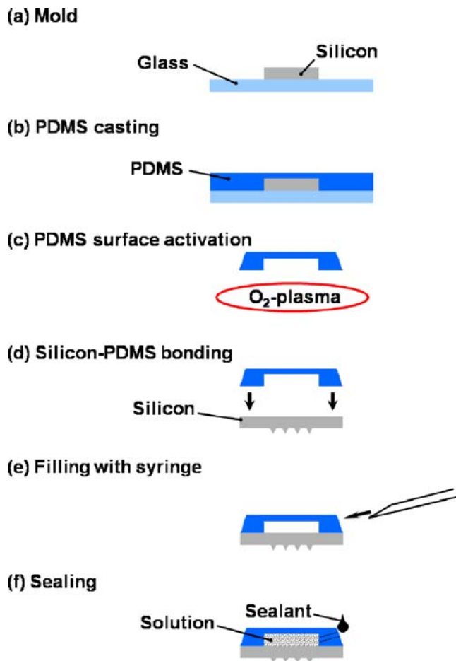
Fig. 2 Process flow for wafer-level PDMS reservoir fabrication and device integration. The silicon mold is prepared (a) and PDMS is poured onto the mold and cured (b). After peeling off and cutting to shape, the PDMS surface is activated using an oxygen plasma (c), allowing the bonding of PDMS and silicon substrate (d). After filling with a conventional syringe (e), the container is resealed (f)
