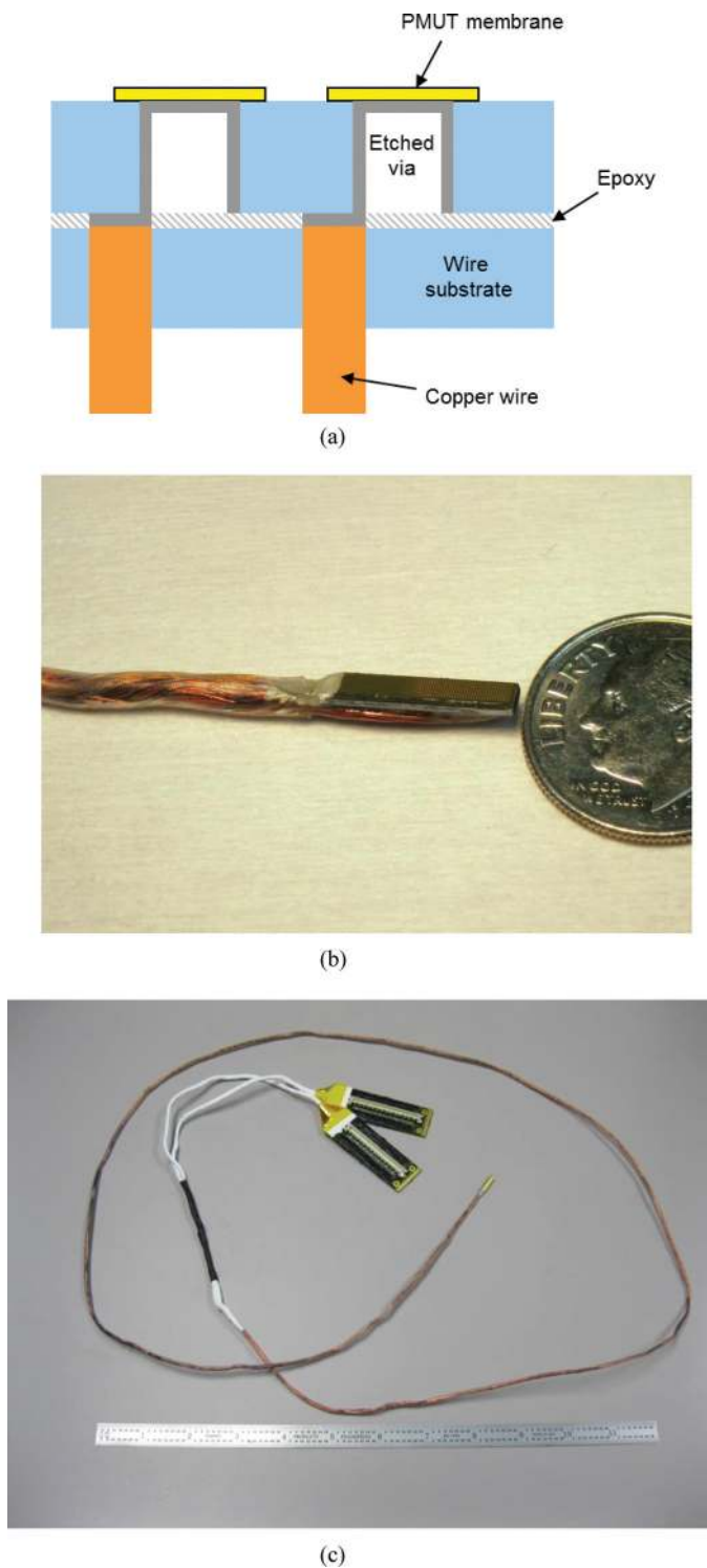
Fig. 3. (a) Cross-sectional schematic of a PMUT array substrate bonded to a signal wire substrate. (b) Photograph of a matrix PMUT array containing 256 active elements ( 64 \times 16 PMUT membranes) interconnected to the distal end of a cable assembly containing 256 signal wires and 128 ground wires. The distal end of the pMUT/termination substrate/wire bundle assembly measured 2.9 mm width \times 2.5 mm height \times 15 mm length. (c) Photograph of the full PMUT-cable assembly measuring 137 cm in length.
