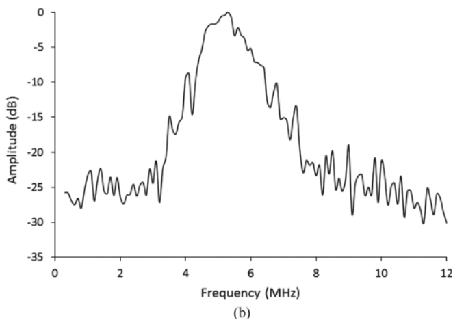
Fig. 8. (a) Transmit pulse from one element of PMUT Array 2 driven with a 3-cycle sine wave at 30 V_{pp} measured by a hydrophone without amplification at 20 mm distance. (b) FFT spectrum of transmit pulse with measured bandwidth of 30%.
