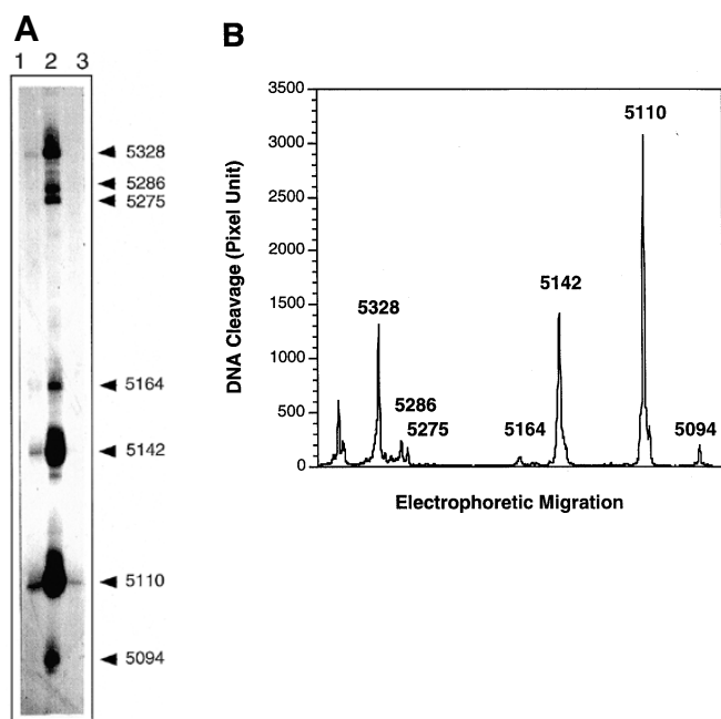
Figure 3. In vivo sequencing of CPT-induced DNA cleavage sites in the 18S rDNA of human colon carcinoma SW620 cells: autoradiography of LM-PCR products. (A) Control DNA from untreated cells was without any signal. Lanes 1 and 2: DNA from cells treated with 0.1 and 10 \mu M CPT, respectively. Lane 3: reversal of CPT-induced DNA breaks. CPT (10 \mu M for 1 h) was removed from cell culture 30 min before DNA extraction. Numbers to the right correspond to genomic positions of the DNA breaks on the lower strand (DDBJ/EMBL/GenBank U13369). Top1 is linked to the nucleotide corresponding to the indicated number. The positions of the cleavage sites at the top of the gel (5275–5328) are \pm 1 nucleotide. (B) Intensity profile of the cleavage sites using the Phosphorimager ImageQuant software (Sunyvale, CA).
