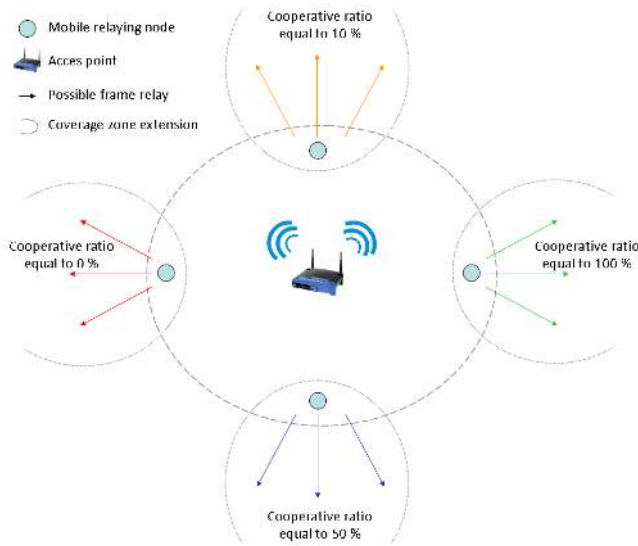
Fig. 6. Simulation setup.
