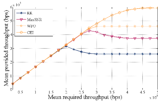
Fig. 11. Relay efficiency.
