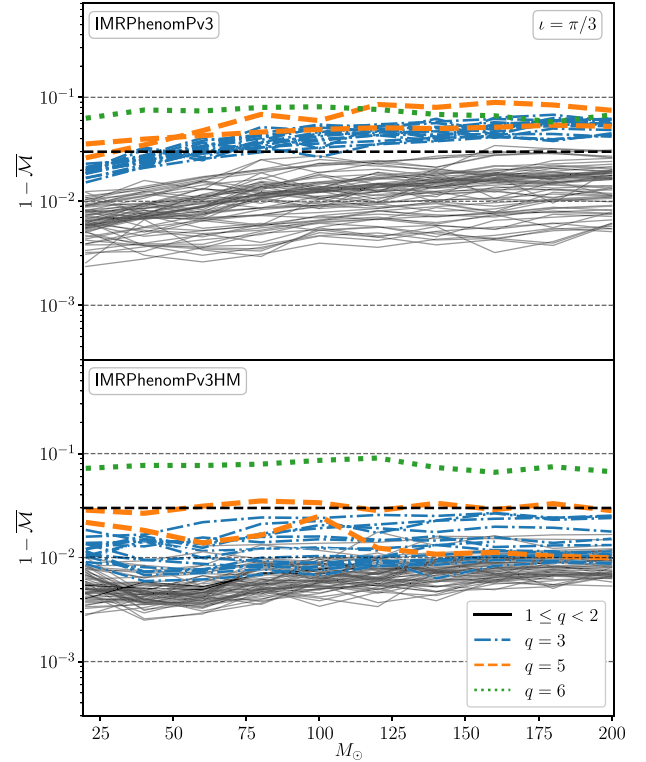
FIG. 2. The results of the comparison between PhenomPv3 (top), PhenomPv3HM (bottom), and the precessing NR simulations from the public SXS catalogue. The figure shows the mismatch average over a reference phase and polarization angle ( 1 - \bar{\mathcal{M}} ) as a function of the total mass for an inclination of \iota = \pi/3 . The worst case is SXS:BBH:0165, a short ( \sim 6 orbits) signal with mass ratio of 1:6 and high precession.
