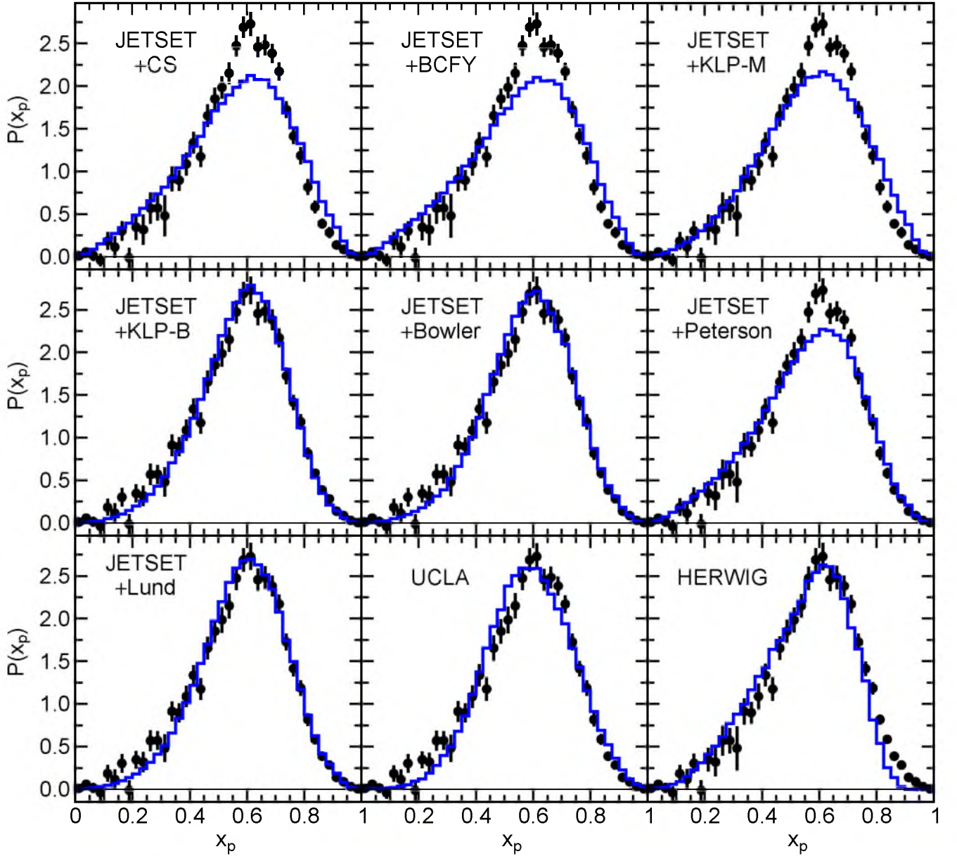
FIG. 8: The A_c^+ x_p distribution (dots) compared with the results of the model tests (histograms) described in the text. The error bars include simulation statistics.
