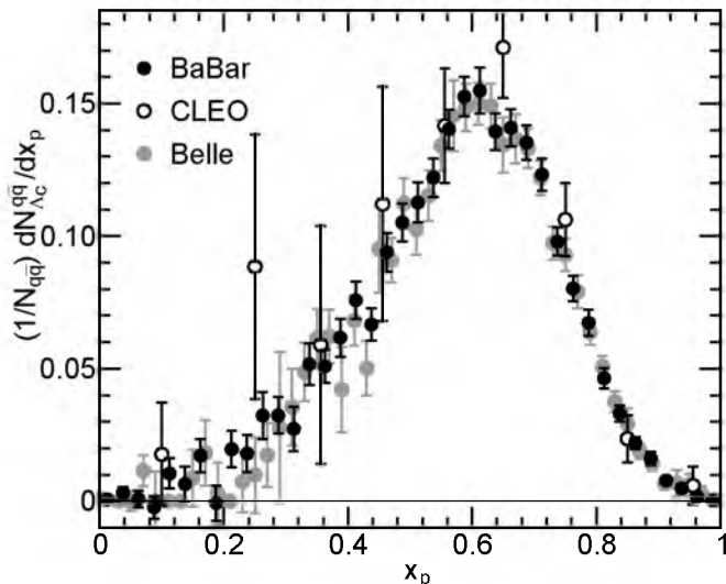
FIG. 6: Differential A_c^+ production rate per e^+e^- \rightarrow q\bar{q} event compared with previous measurements. The error bars include statistics and those systematic errors that affect the shape. Each experiment has a normalization uncertainty of a few percent, and there is an overall 26% uncertainty due to the A_c^+ \rightarrow pK^-\pi^+ branching fraction.
