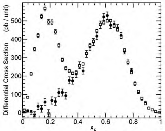
FIG. 5: Differential cross sections for \Lambda_c^+ + \bar{\Lambda}_c^- production in the off-(circles) and on-resonance (open squares) data as functions of x_p . The errors are statistical only.
