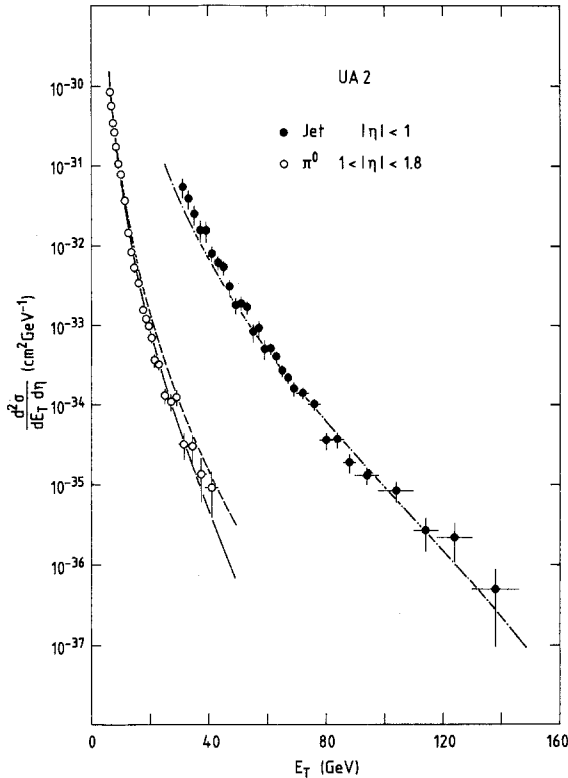
Fig. 12. Comparison of the cross-sections for inclusive jet and \pi^0 productions. The curves are the predicted jet cross-section at \eta=0 (---) and \pi^0 cross-section at \eta=0 (—) and at \eta=1.4 (-·-·-). The calculation uses the structure and fragmentation functions from [17], Q^2 = P_T^2 , \Lambda = 0.31 GeV
