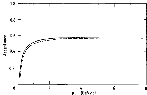
Fig. 4. Acceptance in one hemisphere of the F/B spectrometers for positive (solid line) and negative (dashed line) particles produced at the center of the interaction region
