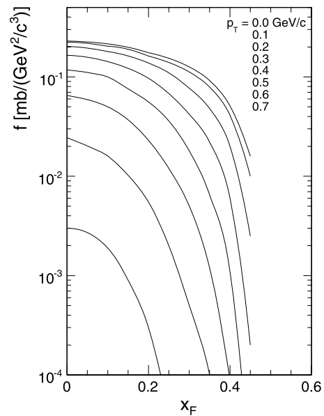
Fig. 57 Interpolated invariant cross sections as a function of x_F for fixed values of p_T
