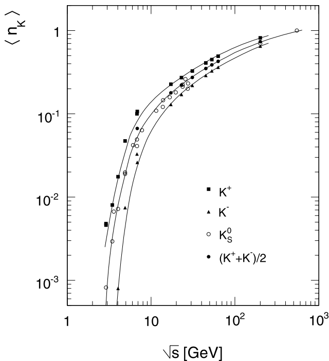
Fig. 130 Total yields \langle n_{K^+} \rangle , \langle n_{K^-} \rangle and \langle n_{K_S^0} \rangle as a function of \sqrt{s} . The full line through the K_S^0 results is an eyeball fit, the lines through the K^+ and K^- data are derived from Fig. 131 below. The full circles in the K_S^0 data correspond to 0.5(\langle n_{K^+} \rangle + \langle n_{K^-} \rangle) established at the corresponding \sqrt{s} values
