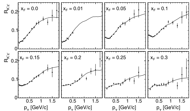
Fig. 32 R_{K^-\pi^-} as a function of p_T at fixed x_F . The lines show the result of the data interpolation, Sect. 6.2
