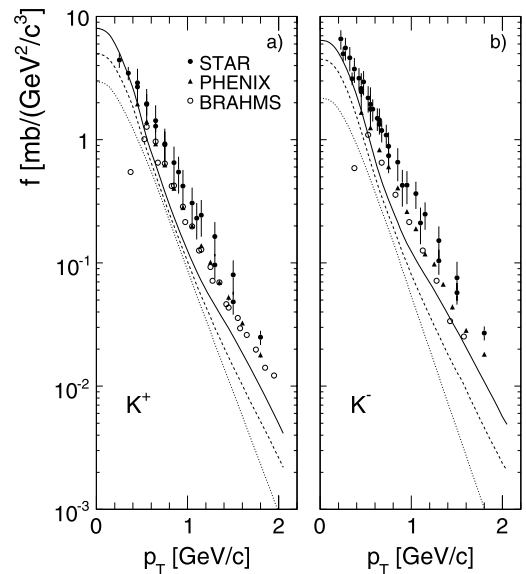
Fig. 96 Invariant kaon cross sections from RHIC at central rapidity and \sqrt{s} = 200 GeV [24–27, 29, 30] as a function of p_T for (a) K^+ and (b) K^- . The corresponding data from NA49 (dotted line), the interpolated data from the ISR at \sqrt{s} = 63 GeV (dashed line) and the extrapolated ISR data at \sqrt{s} = 200 GeV (full line) are also shown
