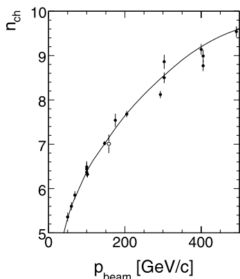
Fig. 55 \langle n_{\text{ch}} \rangle as a function of beam momentum p_{\text{beam}} . The NA49 measurement is indicated with an open circle
