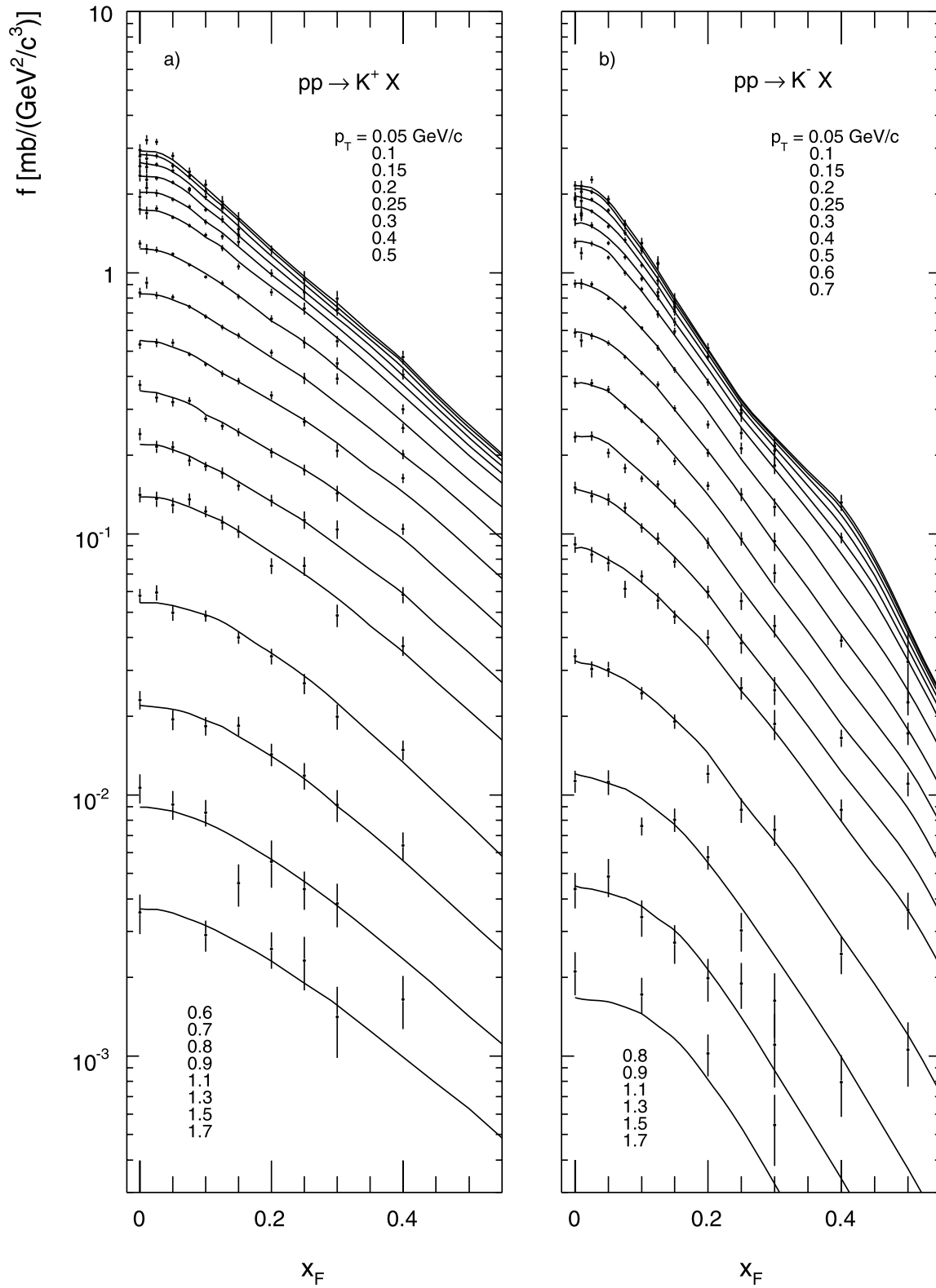
Fig. 22 Double differential invariant cross section f(x_F, p_T) [ \text{mb}/(\text{GeV}^2/c^3) ] as a function of x_F at fixed p_T for (a) K^+ and (b) K^- produced in p+p collisions at 158 GeV/c beam momentum. The lines show the result of the data interpolation, Sect. 6.2
