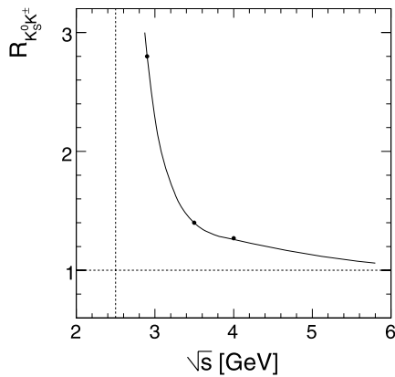
Fig. 59 Ratio R_{K_S^0 K^\pm} between the average charged kaon and K_S^0 yields as a function of \sqrt{s} . The threshold of kaon production is indicated at about \sqrt{s} \sim 2.5 GeV
