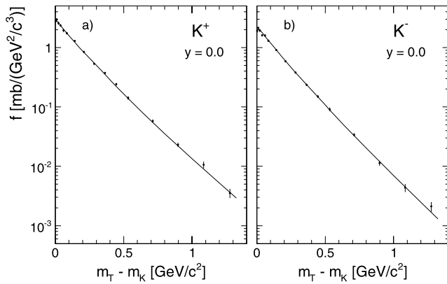
Fig. 24 Invariant cross section as a function of m_T - m_K for (a) K^+ and (b) K^- produced at y = 0.0 . The lines show the result of the data interpolation, Sect. 6.2
