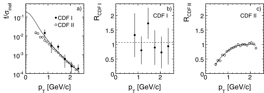
Fig. 109 Comparison of K_S^0 data from CDF with the UA5 fit, (a) cross sections as a function of p_T . CDF I data (full circles), re-normalized CDF II data (open circles); ratios (b) R_{\text{CDF I}} = (\frac{f}{\sigma_{\text{inel}}})_{\text{CDF I}} / (\frac{f}{\sigma_{\text{inel}}})_{\text{UA5 fit}} , (c) R_{\text{CDF II}} = (\frac{f}{\sigma_{\text{inel}}})_{\text{CDF II}} / (\frac{f}{\sigma_{\text{inel}}})_{\text{UA5 fit}} . The mean offset of CDF I data from UA5 fit is indicated in panel (b) with dashed line
