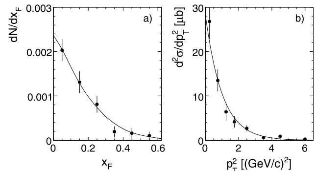
Fig. 126 (a) dn/dx_F as a function of x_F and (b) d\sigma/dp_T^2 as a function of p_T^2 of D(1860)
