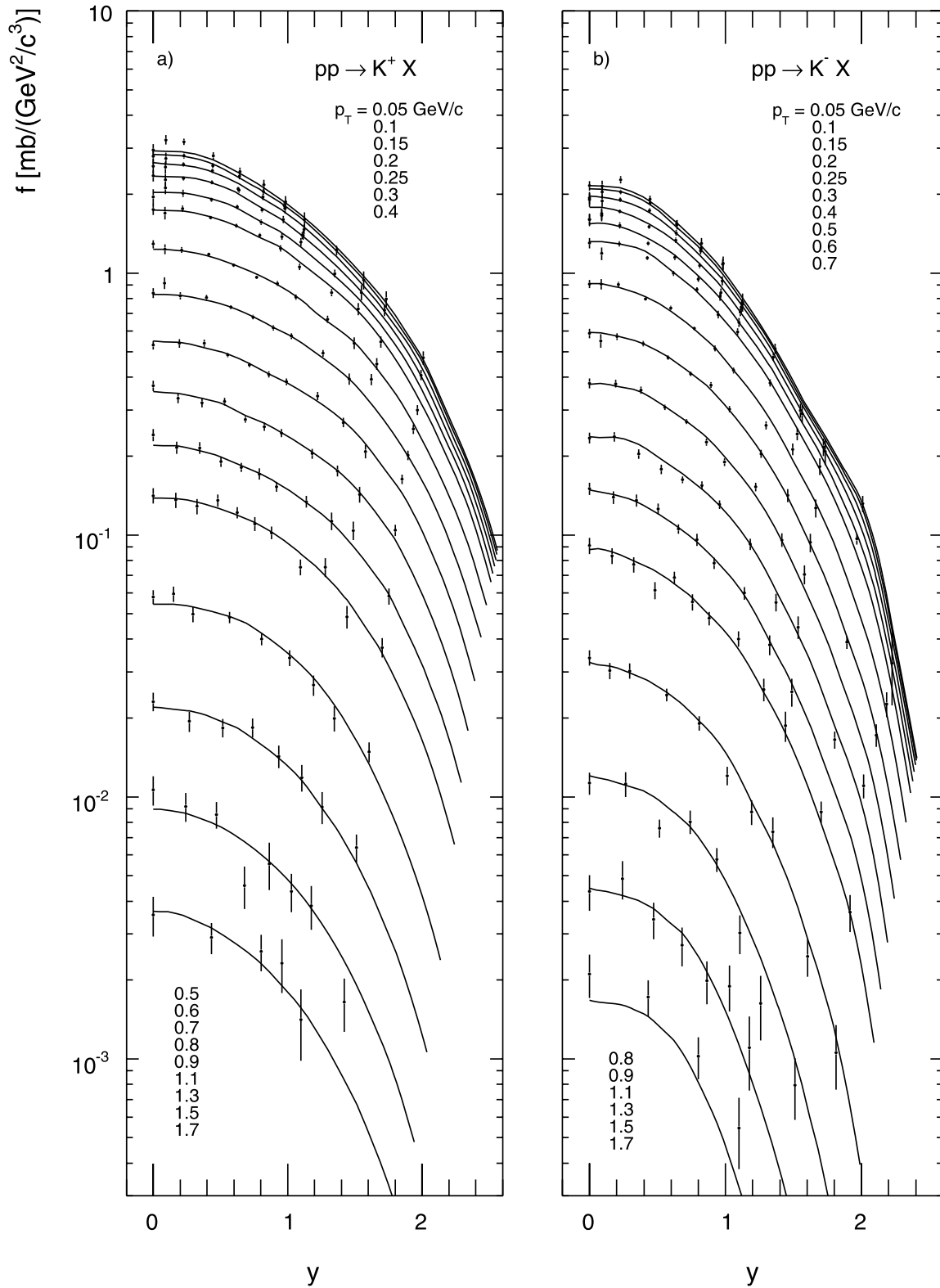
Fig. 23 Double differential invariant cross section f(x_F, p_T) [mb/(GeV 2 /c 3 )] as a function of y at fixed p_T for (a) K^+ and (b) K^- produced in p + p collisions at 158 GeV/c beam momentum. The lines show the result of the data interpolation, Sect. 6.2
