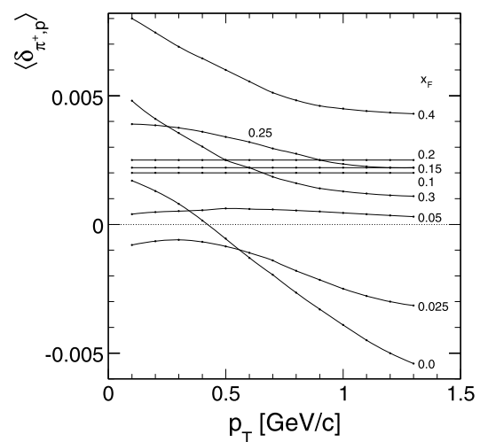
Fig. 7 Mean deviation \langle \delta_{\pi^+, p} \rangle , in units of minimum ionization, of \pi^+ and proton dE/dx with respect to the Bethe–Bloch parametrization as a function of p_T for different values of x_F
