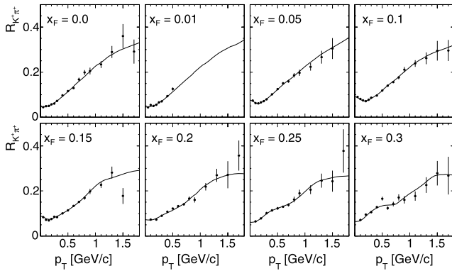
Fig. 29 R_{K^+\pi^+} as a function of p_T at fixed x_F . The lines show the result of the data interpolation, Sect. 6.2
