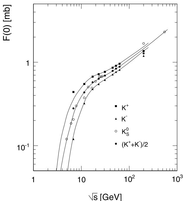
Fig. 134 F(x_F = 0, \sqrt{s}) as a function of \sqrt{s} for K_S^0 (open circles: direct measurements, full circles: obtained as average from K^+ and K^- ), K^+ (squares) and K^- (triangles)
