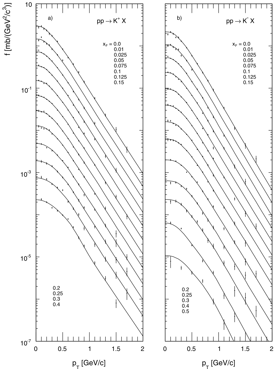
Fig. 21 Double differential invariant cross section f(x_F, p_T) [\text{mb}/(\text{GeV}^2/c^3)] as a function of p_T at fixed x_F for (a) K^+ and (b) K^- produced in p + p collisions at 158 \text{GeV}/c beam momentum. The dis-
