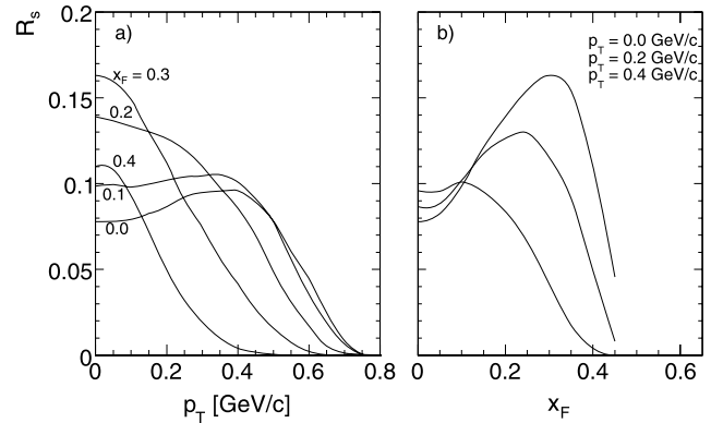
Fig. 60 Ratio R_s as a function of (a) p_T at fixed x_F and (b) x_F at fixed p_T
