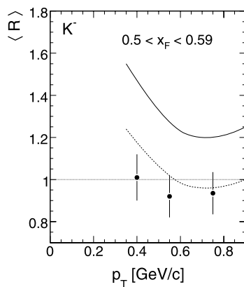
Fig. 84 Ratio \langle R \rangle between [17] and NA49 K^- as a function of p_T averaged over the x_F region from 0.5 to 0.59. The full line gives the behaviour at x_F = 0 , the broken line shows the consequence of a 20% normalization error
