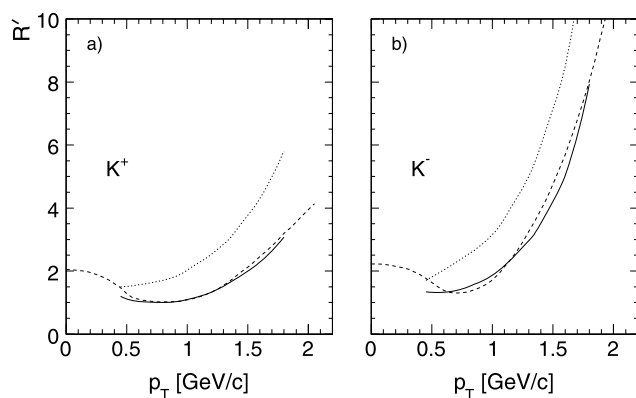
Fig. 100 Ratios R' as functions of p_T , for the data from PHENIX [27] divided by 1.3 \cdot \epsilon (full line) and the extrapolated ISR data at \sqrt{s} = 200 GeV (dashed line). Panel (a) for K^+ , (b) for K^-
