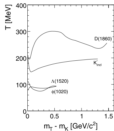
Fig. 129 Inverse slopes of K^- from the decay of \phi(1020) , \Lambda(1520) and D(1860) as a function of m_T - m_K . The result for inclusive K^- production is also shown
