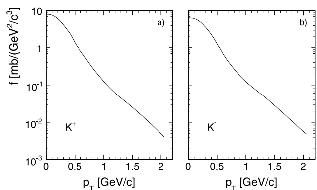
Fig. 92 f(x_F = 0, p_T) as a function of p_T extrapolated to \sqrt{s} = 200 GeV for (a) K^+ , (b) K^-
