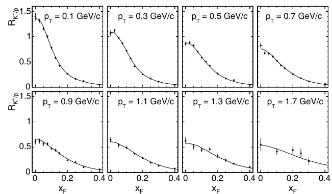
Fig. 36 R_{K^+p} as a function of x_F at fixed p_T . The lines show the result of the data interpolation, Sect. 6.2
