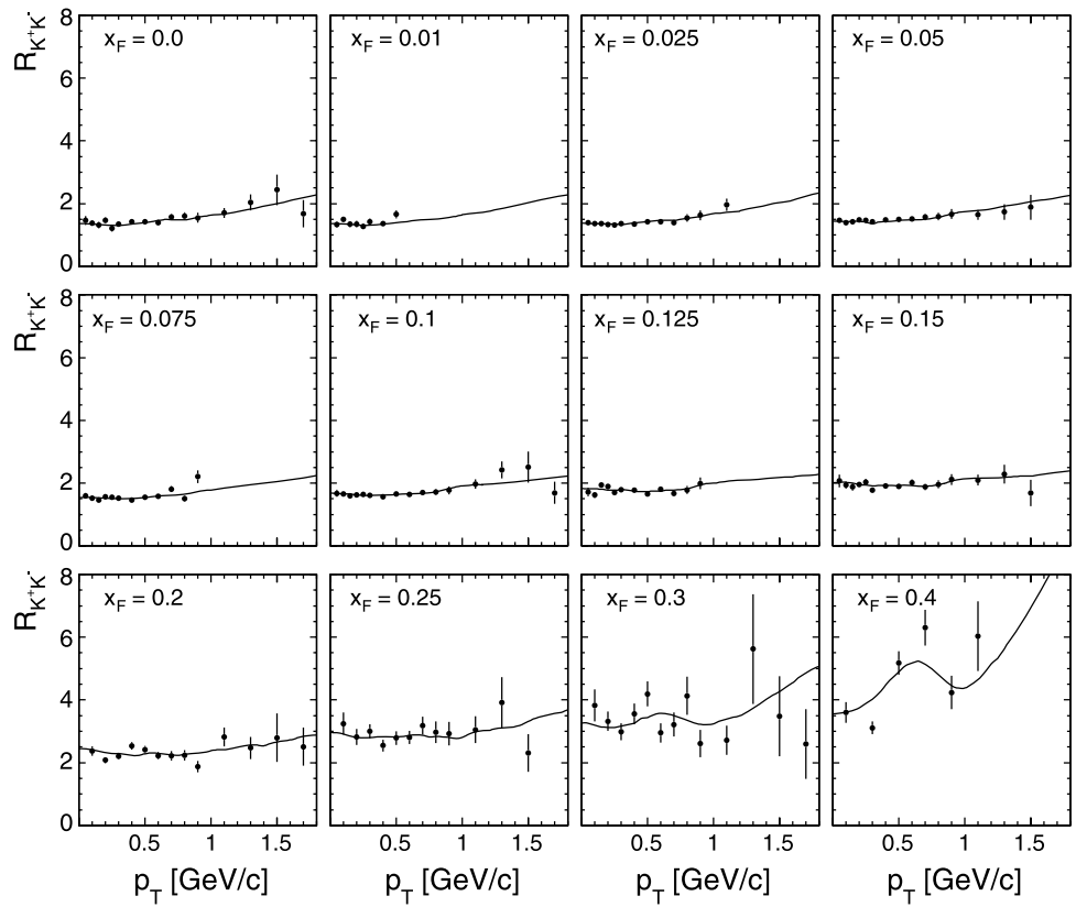
Fig. 27 R_{K^+K^-} as a function of p_T at fixed x_F . The lines show the result of the data interpolation, Sect. 6.2
