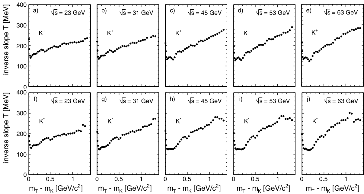
Fig. 74 Inverse slopes of the interpolated m_T distributions as function of m_T - m_K for the 5 ISR energies and for K^+ (panels (a) to (e)) and for K^- (panels (f) to (j))
