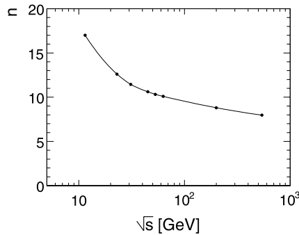
Fig. 115 Fitted exponent n as a function of \sqrt{s} . The full line is shown to guide the eye
