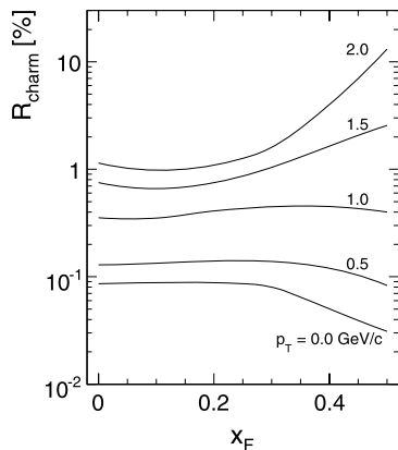
Fig. 128 R_{\text{charm}} as a function of x_F for fixed values of p_T , in %
