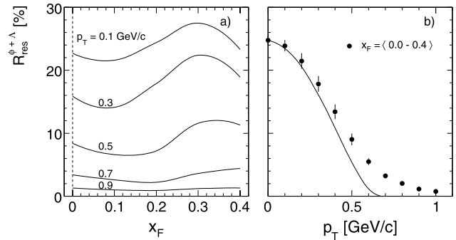
Fig. 125 Ratio R_{\text{res}}^{\phi+\Lambda} = K_{\phi+\Lambda}^{-} / K_{\text{incl}}^{-} (a) as a function of x_F for different p_T and (b) as a function of p_T averaged over the x_F range 0 < x_F < 0.4 . In panel (b) the error bars give the variation with x_F around the average. The full line represents the relative increase of the K^{-} cross section as a function of \sqrt{s} , Fig. 73b, normalized at p_T = 0 GeV/c
