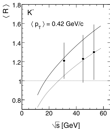
Fig. 82 Ratio \langle R \rangle between [15] and NA49 averaged over the intervals 0.2 < p_T < 0.7 GeV/c and 0.15 < x_F < 0.5 as a function of \sqrt{s} . Full line: behaviour at x_F = 0 , broken line: 15% normalization error
