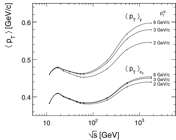
Fig. 117 \langle p_T \rangle_{x_F} at x_F = 0 and \langle p_T \rangle_y at y = 0 as a function of \sqrt{s} for different values of the upper integration limit from 2 to 6 GeV/c
