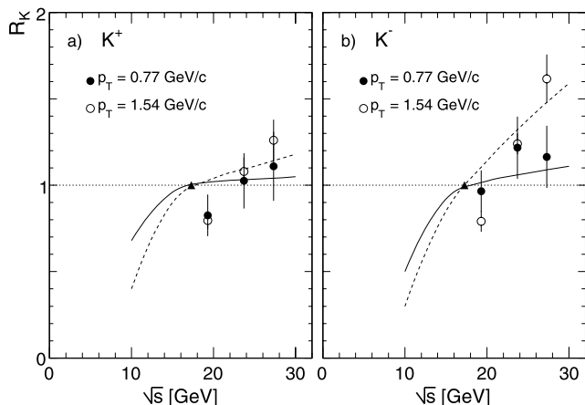
Fig. 46 The cross section ratios between the data from [12] and NA49 as a function of \sqrt{s} for two values of p_T for (a) K^+ and (b) K^- . In both of the panels the NA49 point is indicated with full triangle . The full and dashed lines represent the result of the s -dependence at x_F = 0 established in Sect. 10 below at p_T = 0.77 and 1.54 GeV/c, respectively
