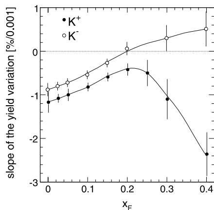
Fig. 10 Slope of the yield variation given in % per assumed kaon shift of 0.001 for K^+ and K^- as a function of x_F , averaged over p_T
