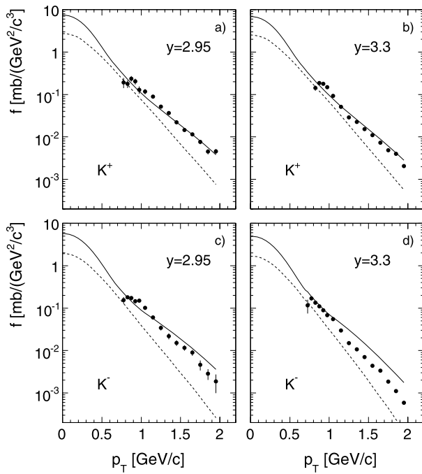
Fig. 102 Invariant cross sections as a function of p_T for rapidity 2.95 and 3.3 for K^+ (panels (a) and (b)) and K^- (panels (c) and (d)), respectively. Also shown are the NA49 data ( dashed lines ) and the extrapolated ISR data ( full lines ) at these rapidities
