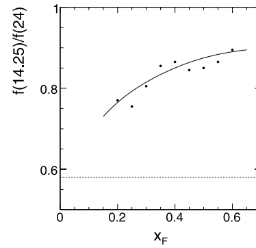
Fig. 67 f(14.25 \text{ GeV}/c)/f(24 \text{ GeV}/c) as a function of x_F
