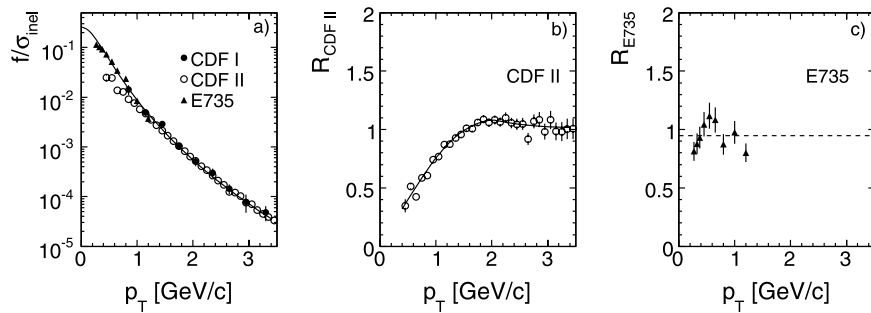
Fig. 111 Kaon data at \sqrt{s} = 1800 GeV; (a) full line fit to the CDF I data [78]. Full circles: CDF I data. Open circles: CDF II data re-normalized to the CDF I fit at p_T = 1.55 GeV/c. Triangles: E735 data re-normalized to the CDF I fit. (b) Ratio between the re-normalized
