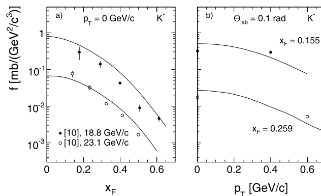
Fig. 64 K^- comparison Dekkers [10] and Allaby (a) K^- , p_T = 0 \text{ GeV}/c as a function of x_F . Full lines [7, 8] extrapolation at 19.2 and 24 \text{GeV}/c beam momentum, data points from [10] at 18.8 and 23.1 \text{GeV}/c (b) Dekkers data and Allaby interpolation at 18.8
