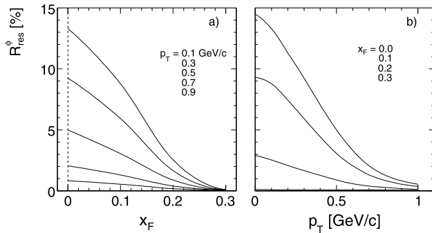
Fig. 122 Ratio R_{\text{res}}^{\phi} = K_{\phi}^{-} / K_{\text{incl}}^{-} as a function of (a) x_F for different p_T and (b) p_T for different x_F
