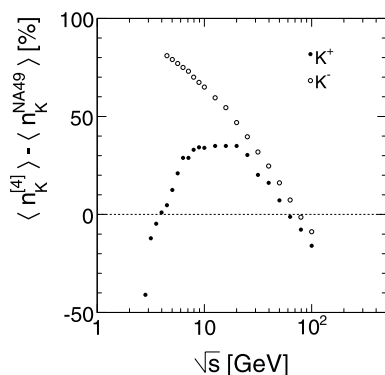
Fig. 133 Relative deviations between the present study of charged kaon yields and [4] in percent as a function of \sqrt{s}
