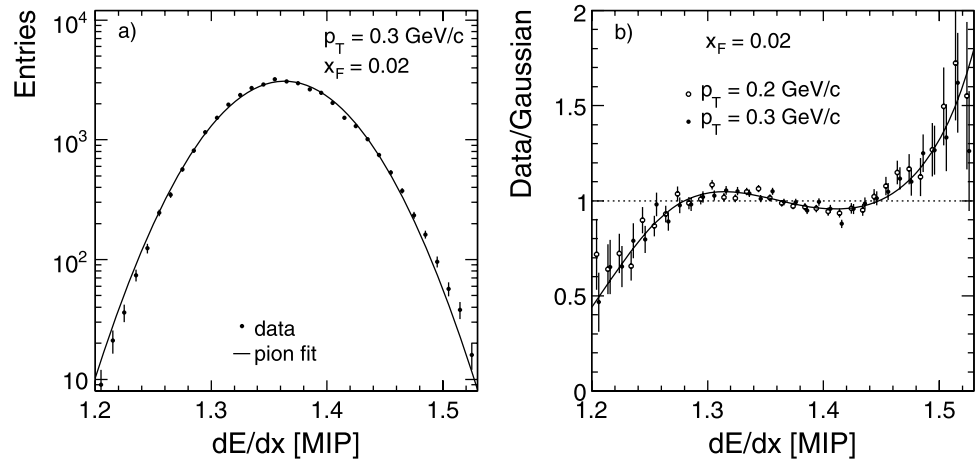
Fig. 6 (a) Conventional Gaussian fit of the MTPC dE/dx distribution, for tracks with pion selection using the VTTPC dE/dx ; (b) ratio of data and fit function
