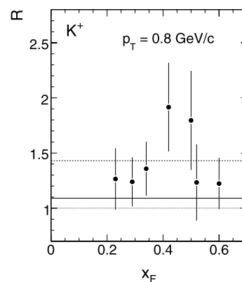
Fig. 86 Ratio R between [18] and NA49 for K^+ as a function of x_F at p_T = 0.8 GeV/c and \sqrt{s} = 45 GeV. The dashed line shows the mean ratio of the measured points and the full line shows the ratio at x_F = 0
