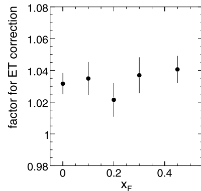
Fig. 13 Empty target correction for K^+ and K^- as a function of x_F , averaged over p_T
