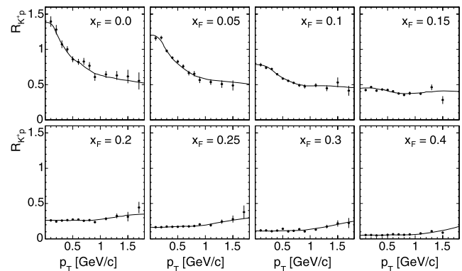
Fig. 35 R_{K^+p} as a function of p_T at fixed x_F . The lines show the result of the data interpolation, Sect. 6.2
