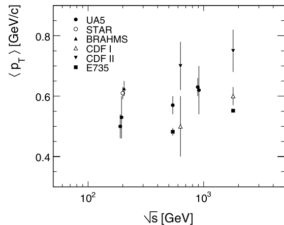
Fig. 112 \langle p_T \rangle in the \sqrt{s} range from 200 to 1800 GeV from different experiments
