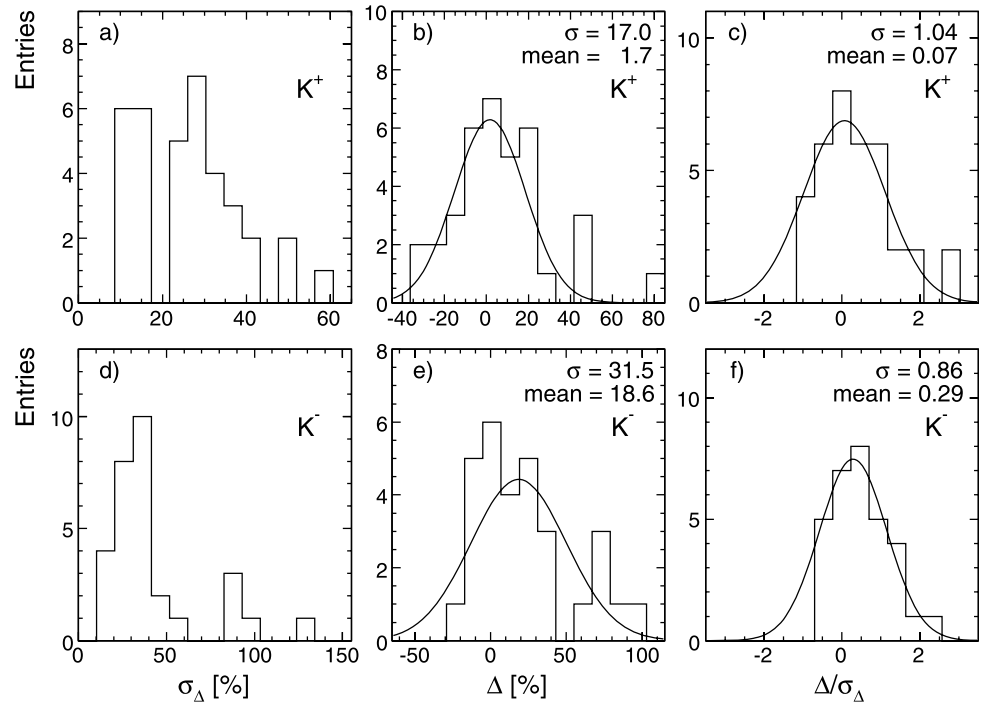
Fig. 42 Statistical analysis of the difference between the measurements of [13] and NA49 for K^+ (upper three panels) and K^- (lower three panels): (a) and (d) error of the difference of the measurements; (b) and (e) difference of the measurements; (c) and (f) difference divided by the error
