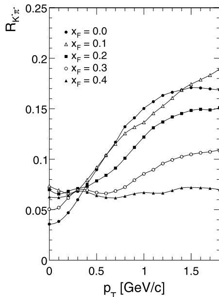
Fig. 34 R_{K^-\pi^-} as a function of p_T for different x_F
