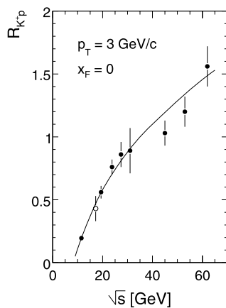
Fig. 38 s -dependence of R_{K^+p} at p_T = 3 GeV/c and x_F = 0 . The open circle corresponds to the NA49 extrapolation, Fig. 37
