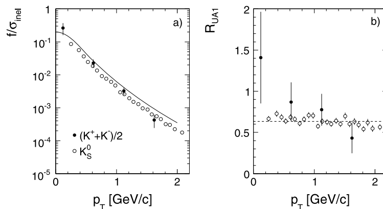
Fig. 106 UA5 data at \sqrt{s} = 540 GeV. The full line corresponds to the fit described in the text
