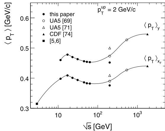
Fig. 114 \langle p_T \rangle_{x_F} at x_F = 0 and \langle p_T \rangle_y at y = 0 as a function of \sqrt{s} . The lines are drawn to guide the eye
