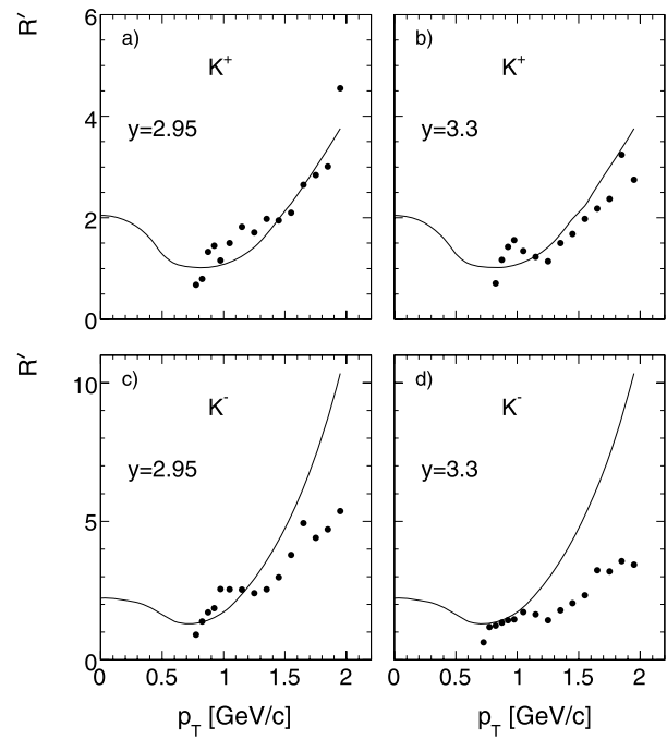
Fig. 103 Ratio R' of kaon densities per inelastic event as a function of p_T for K^+ (panels (a) and (b)) and K^- (panels (c) and (d)). The ratios R' corresponding to the extrapolated ISR data are shown as the full lines
