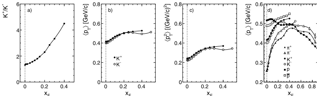
Fig. 51 (a) K^+/K^- ratio, (b) mean p_T , and (c) mean p_T^2 as a function of x_F for K^+ and K^- produced in p + p interactions at 158 GeV/c; (d) mean p_T for \pi^+ , \pi^- , K^+ , K^- , p , \bar{p} on an enlarged vertical scale
