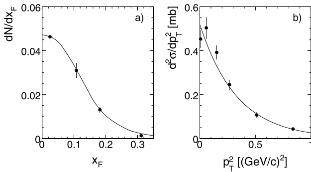
Fig. 121 (a) x_F and (b) p_T^2 distributions of \phi
