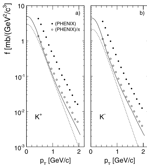
Fig. 98 Invariant kaon cross sections at \sqrt{s} = 62.4 \text{ GeV} from PHENIX [28], for (a) K^+ and (b) K^- , as a function of p_T . The original data points (full points) and the data divided by \pi (open points) are indicated. The data from the ISR [22, 23] at \sqrt{s} = 63 \text{ GeV} are also shown, together with the NA49 data, as the full and dashed lines, respectively
