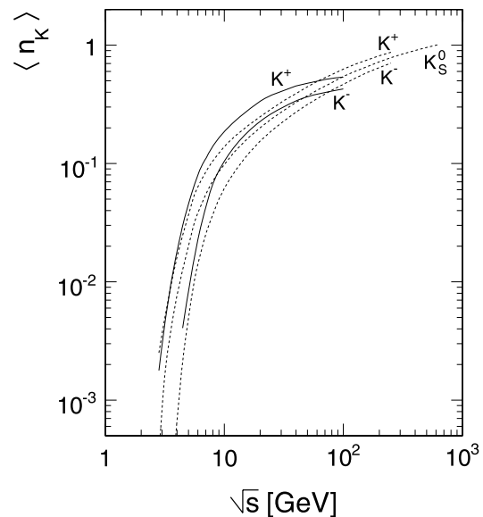
Fig. 132 \langle n_{K^+} \rangle and \langle n_{K^-} \rangle from [4] as a function of \sqrt{s} , full lines, compared to the interpolated K^+ , K^- and K_S^0 yields Fig. 130 (broken lines)
