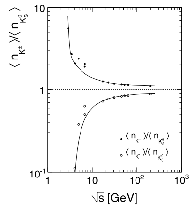
Fig. 131 Ratios \langle n_{K^+} \rangle / \langle n_{K_S^0} \rangle and \langle n_{K^-} \rangle / \langle n_{K_S^0} \rangle as a function of \sqrt{s} . The full lines are eyeball fits through the data at \sqrt{s} < 4.9 GeV and \sqrt{s} > 6.8 GeV
