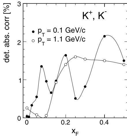
Fig. 16 Correction due to the absorption of produced kaons in the downstream detector material as a function of x_F for two p_T values. The lines are shown to guide the eye
