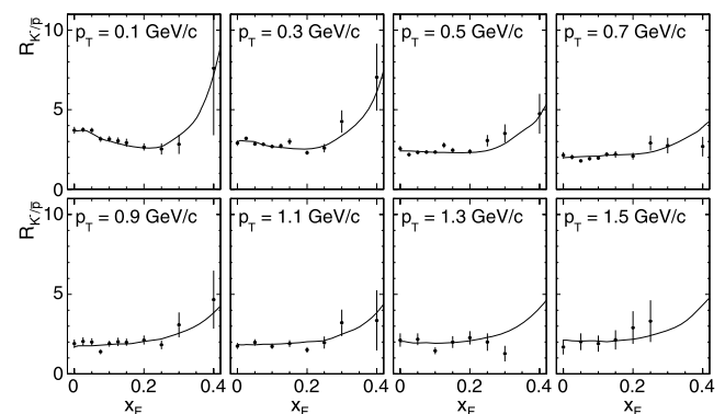
Fig. 40 R_{K^+p} as a function of x_F at fixed p_T . The lines show the result of the data interpolation, Sect. 6.2
