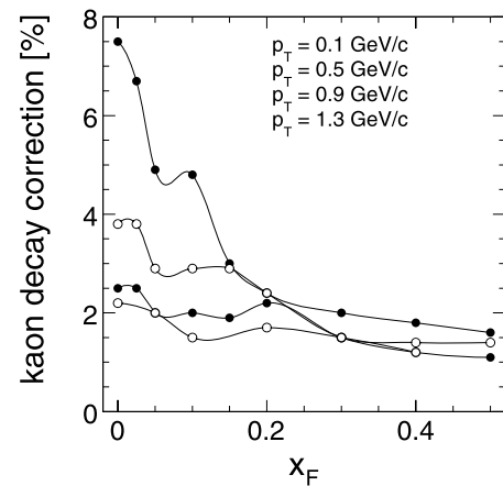
Fig. 17 Decay correction as a function of x_F at different p_T values. The lines are shown to guide the eye
