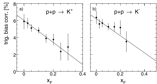
Fig. 14 Trigger bias correction as a function of x_F for (a) K^+ and (b) K^- . The lines correspond to the parametrization of the correction
