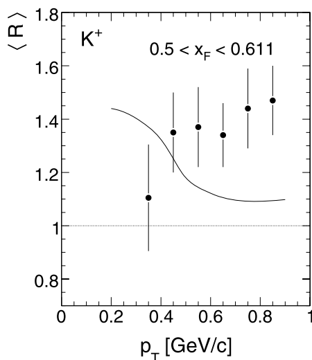
Fig. 88 Ratio \langle R \rangle between [17] and NA49, averaged over x_F , as a function of p_T . The p_T dependence at x_F = 0 is given as the full line
