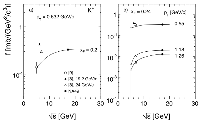
Fig. 66 K^+ comparison as a function of \sqrt{s} (a) p_T = 0.632 GeV/c for x_F = 0.2 (b) x_F = 0.24 for p_T = 0.55, 1.18 and 1.26 GeV/c
