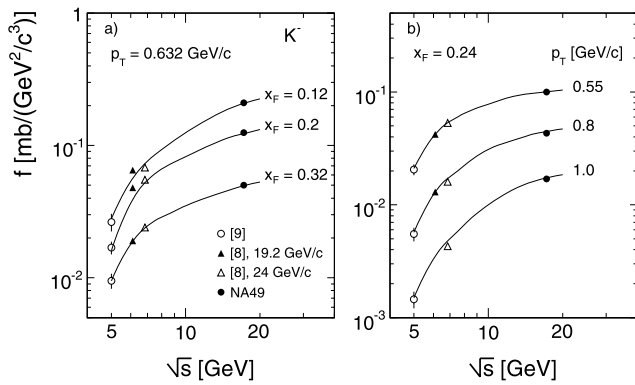
Fig. 65 K^- comparison as a function of \sqrt{s} , (a) p_T = 0.632 GeV/c for x_F = 0.12, 0.2 and 0.32 (b) x_F = 0.24 for p_T = 0.55, 0.8 and 1.0 GeV/c
