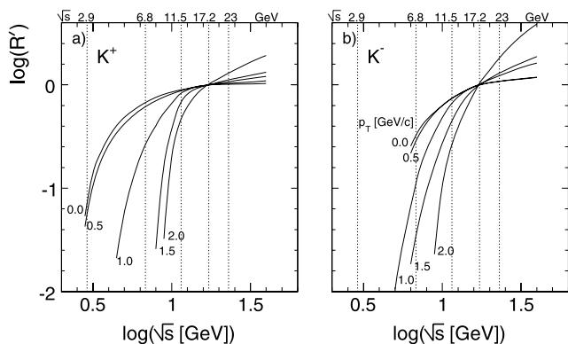
Fig. 91 R' as a function of \sqrt{s} for (a) K^+ and (b) K^- at p_T = 0, 0.5, 1, 1.5, 2 GeV/c. The values of \sqrt{s} are indicated with dotted lines
