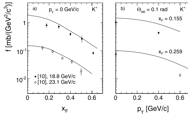
Fig. 63 K^+ comparison Dekkers [10] and Allaby (a) K^+ , p_T = 0 \text{ GeV}/c as a function of x_F . Full lines [7, 8] extrapolation at 19.2 and 24 \text{GeV}/c beam momentum, data points from [10] at 18.8 and 23.1 \text{GeV}/c (b) Dekkers data and Allaby interpolation at 18.8
