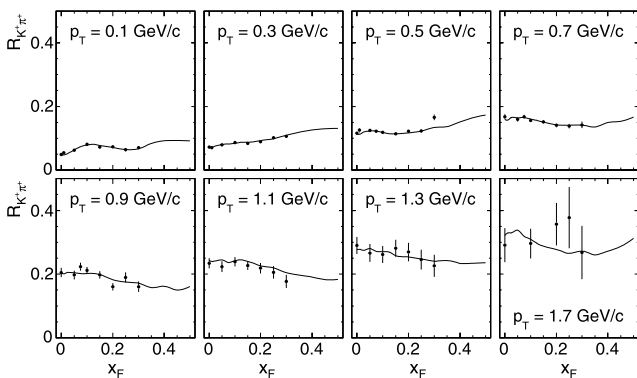
Fig. 30 R_{K^+\pi^+} as a function of x_F at fixed p_T . The lines show the result of the data interpolation, Sect. 6.2
