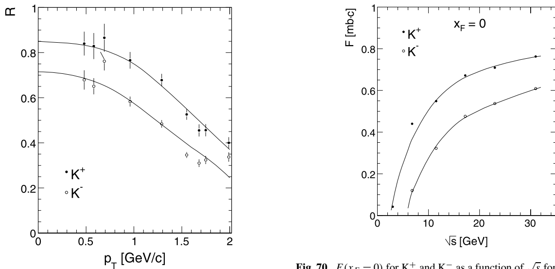
Fig. 69 Cross section ratio R of [11] to NA49 for K^+ and K^-
