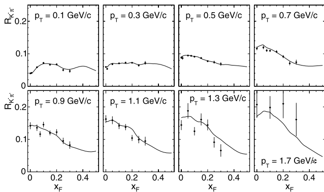
Fig. 33 R_{K^-\pi^-} as a function of x_F at fixed p_T . The lines show the result of the data interpolation, Sect. 6.2
