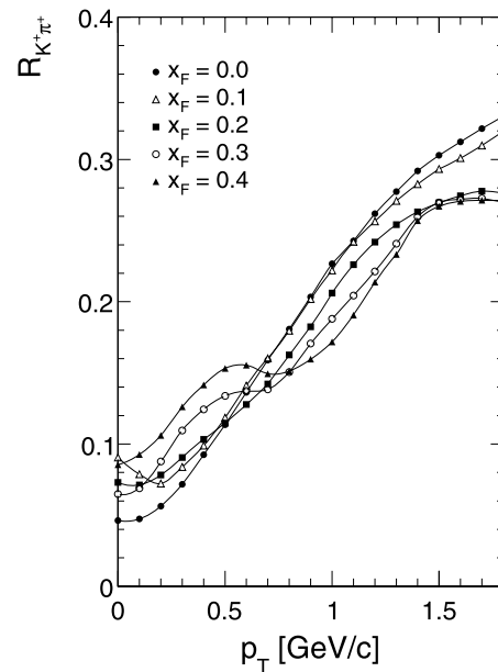
Fig. 31 R_{K^+\pi^+} as a function of p_T for different x_F
