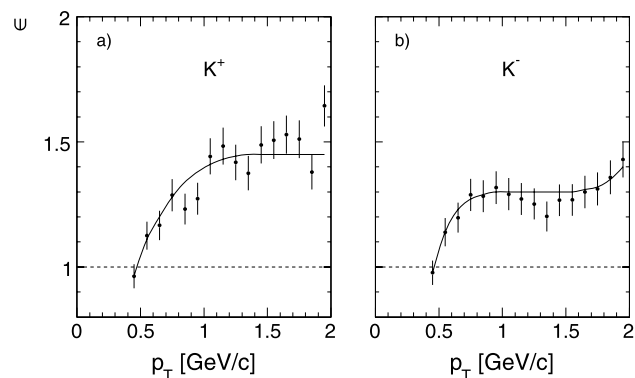
Fig. 99 Cross section ratio \epsilon(p_T) as a function of p_T for (a) K^+ and (b) K^- . The full lines give a representation of \epsilon as a constant offset at p_T > 1 \text{ GeV}/c combined with an efficiency loss towards lower p_T
