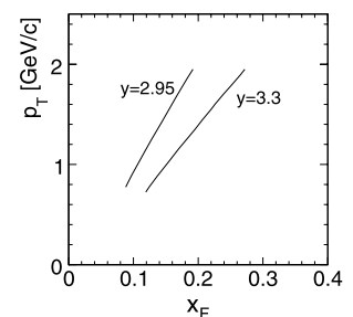
Fig. 101 Correlation between x_F and p_T for the two rapidities 2.95 and 3.3 of [31] at \sqrt{s} = 200 GeV/c
