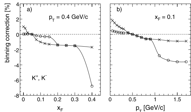
Fig. 18 Binning correction, (a) as a function of x_F for p_T = 0.4 GeV/c and (b) as a function of p_T for x_F = 0.1 . The crosses represent the corrections for fixed values of \delta x_F = 0.05 and \delta p_T = 0.1 GeV/c, respectively, and the open circles give the corrections for the used bin widths. The lines are shown to guide the eye
