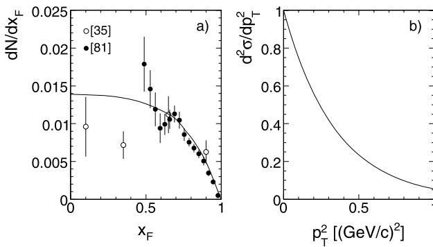
Fig. 123 (a) x_F and (b) p_T^2 distributions of \Lambda(1520)
