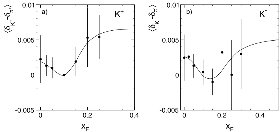
Fig. 8 Mean deviations in units of minimum ionization of (a) K^+ and (b) K^- with respect to the pion position \langle \delta_{K^\pm} - \delta_{\pi^\pm} \rangle as a function of x_F , averaged over p_T
