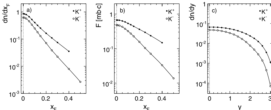
Fig. 50 Integrated distributions of K^+ and K^- produced in p + p interactions at 158 GeV/c: (a) density distribution dn/dx_F as a function of x_F ; (b) invariant cross section F as a function of x_F ; (c) density distribution dn/dy as a function of y
