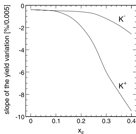
Fig. 11 Slope of the yield variation given in % per assumed change of \sigma_{\text{rel}} of 0.005 for K^+ and K^- as a function of x_F , averaged over p_T
