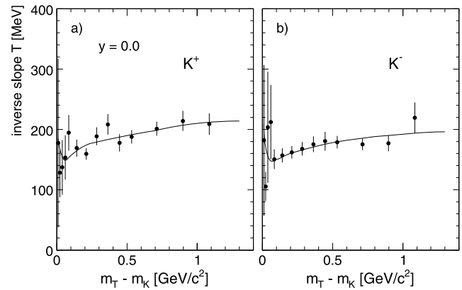
Fig. 25 Local inverse slope of the m_T distribution as a function of m_T - m_K for (a) K^+ and (b) K^- . The lines correspond to the data interpolation, Sect. 6.2
