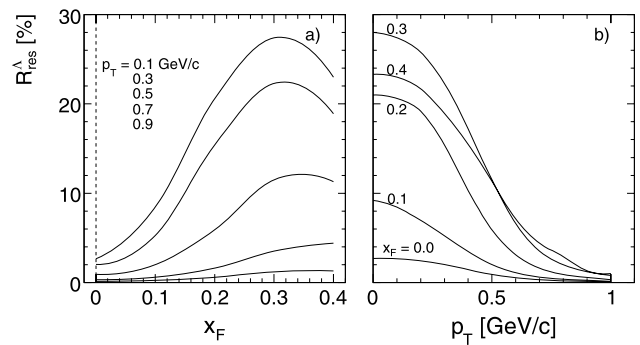
Fig. 124 Ratio R_{\text{res}}^{\Lambda} = K_{\Lambda}^{-} / K_{\text{incl}}^{-} as a function of (a) x_F for different p_T and (b) p_T for different x_F
