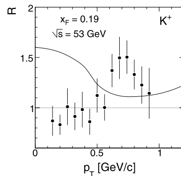
Fig. 85 Ratio R between [16] and NA49 for K^+ at x_F = 0.19 as a function of p_T . The full line gives the behaviour at x_F = 0
