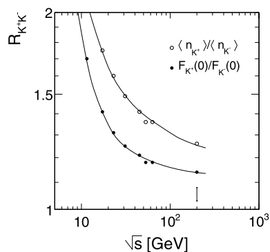
Fig. 136 R_{K^+K^-} ratios for total yields (open circles) and F(x_F = 0) (closed circles) as a function of \sqrt{s} . The error bar at \sqrt{s} = 200 GeV marks the range of F_{K^+}(0)/F_{K^-}(0) of published results by the RHIC experiments
