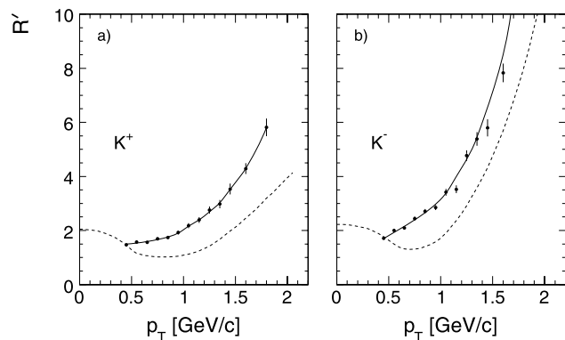
Fig. 97 Ratios R' , (30), as functions of p_T , for the data from PHENIX [27] (full line) and the extrapolated ISR data at \sqrt{s} = 200 \text{ GeV} (dashed line). Panel (a) for K^+ , (b) for K^-
