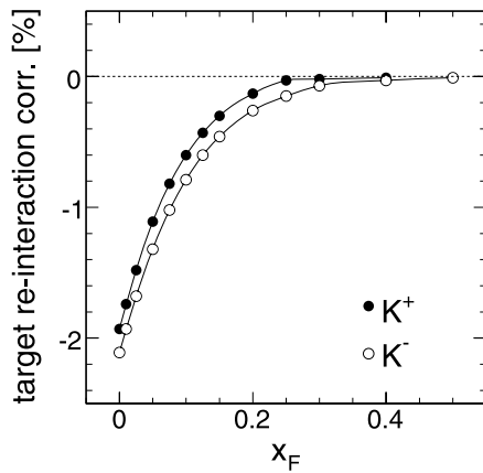
Fig. 15 Target re-interaction correction as a function of x_F
