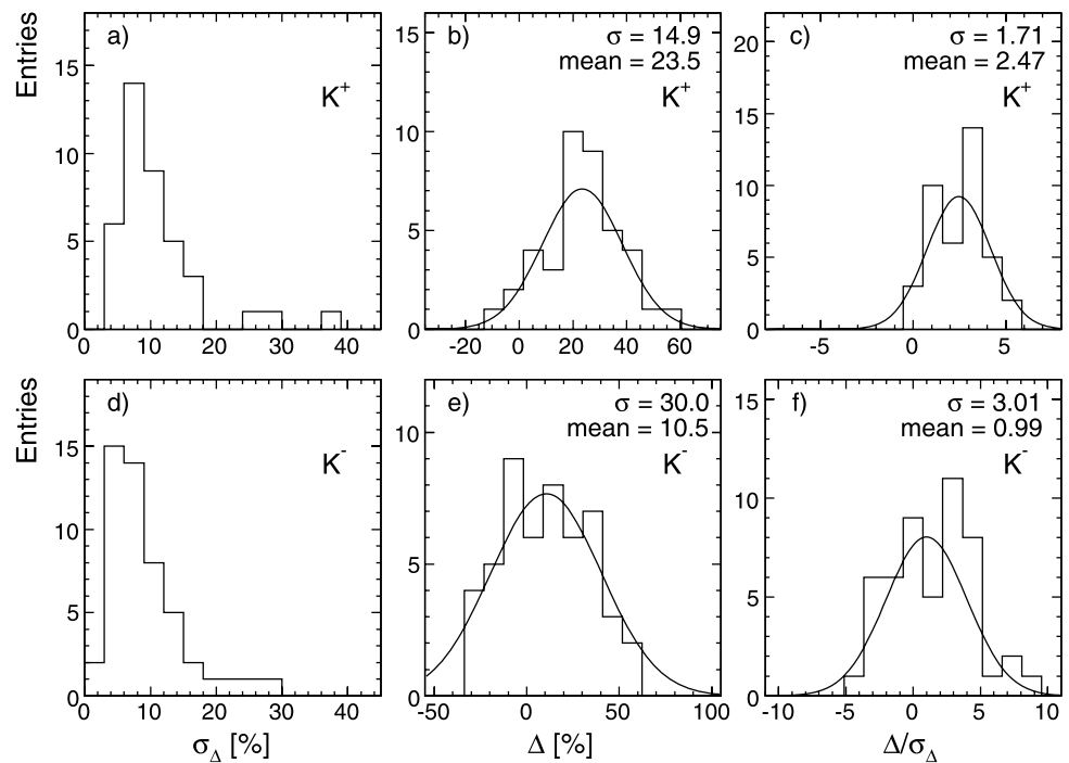
Fig. 44 Statistical analysis of the difference between the measurements of [14] and NA49 for K^+ (upper three panels) and K^- (lower three panels): (a) and (d) error of the difference of the measurements; (b) and (e) difference of the measurements; (c) and (f) difference divided by the error
