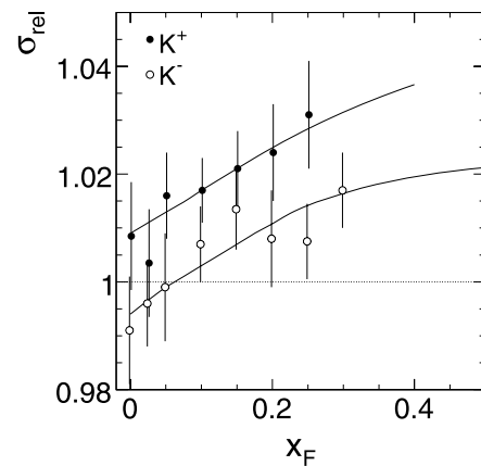
Fig. 9 Relative rms width \sigma_{rel} as a function of x_F for K^+ and K^- , averaged over p_T
