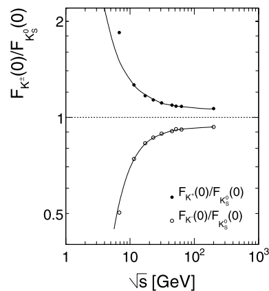
Fig. 135 Ratio between K^+ and interpolated K_S^0 data (full circles) and between K^- and interpolated K_S^0 data (open circles) as a function of \sqrt{s}
