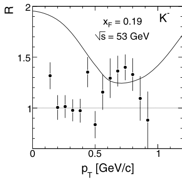
Fig. 83 Ratio R between [16] and NA49 for K^- at x_F = 0.19 as a function of p_T . The full line gives the behaviour at x_F = 0
