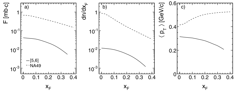
Fig. 58 p_T integrated (a) F , (b) dn/dx_F and (c) \langle p_T \rangle distributions as a function of x_F . The results obtained at \sqrt{s} = 17.2 GeV (dashed lines) are also shown for comparison
