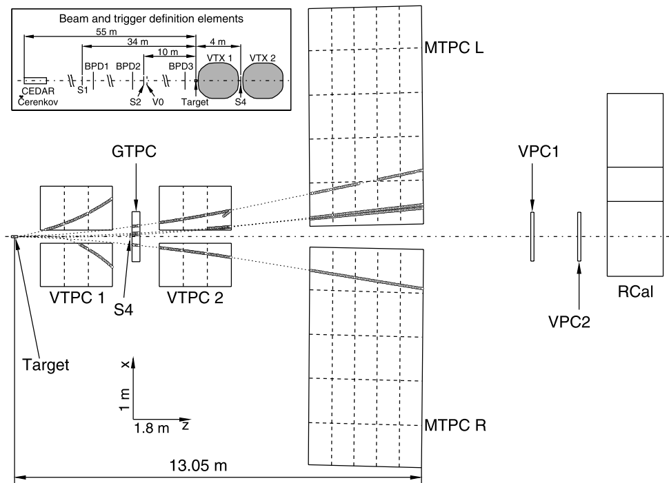
Fig. 3 NA49 detector layout and real tracks of a typical mean multiplicity p + p event. The open circles are the points registered in the TPC's, the dotted lines are the interpolated trajectories between the track segments and the extrapolations to the event vertex in the LH_2 target. The beam and trigger definition counters are presented in the inset
