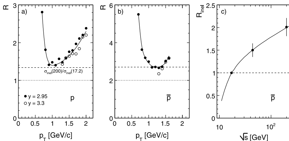
Fig. 54 Ratio R between BRAHMS and NA49 invariant cross sections as a function of p_T at two rapidity values for (a) protons and (b) anti-protons; (c) R_{\text{inel}} as function of \sqrt{s} for \bar{p} including measurements from the ISR [23]. For the BRAHMS data the p_T range from 1 to 1.5 GeV/c is used. The ratio of inelastic cross sections \sigma_{\text{inel}}(200)/\sigma_{\text{inel}}(17.2) is indicated in panel (a) with a dashed line
