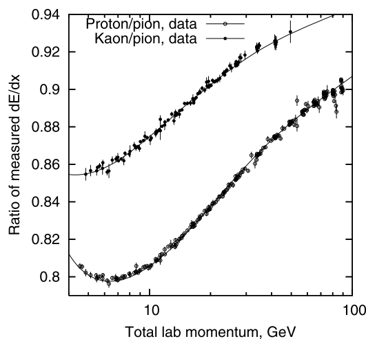
Fig. 10 Ratios of the measured truncated mean dE/dx , protons and kaons relative to pions. The lines correspond to the calibrated Argon Bethe–Bloch curve, the data points are individual fits on the p+p data
