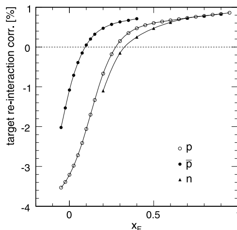
Fig. 15 Target re-interaction correction
