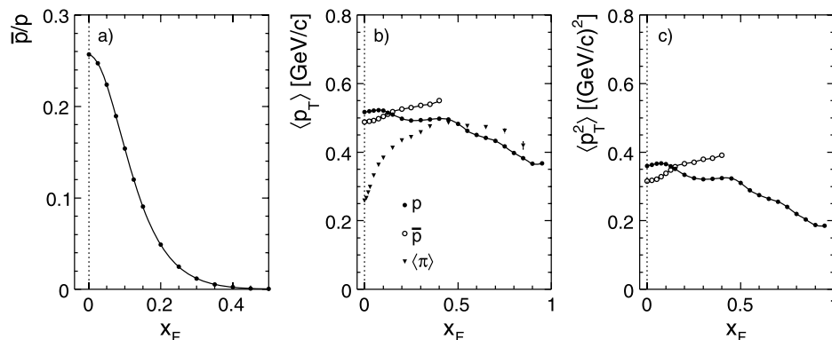
Fig. 56 (a) \bar{p}/p ratio, (b) mean p_T , and (c) mean p_T^2 as a function of x_F for p and \bar{p} produced in p+p interactions at 158 GeV/c. In panel (b) the mean p_T of (\pi) is also shown
