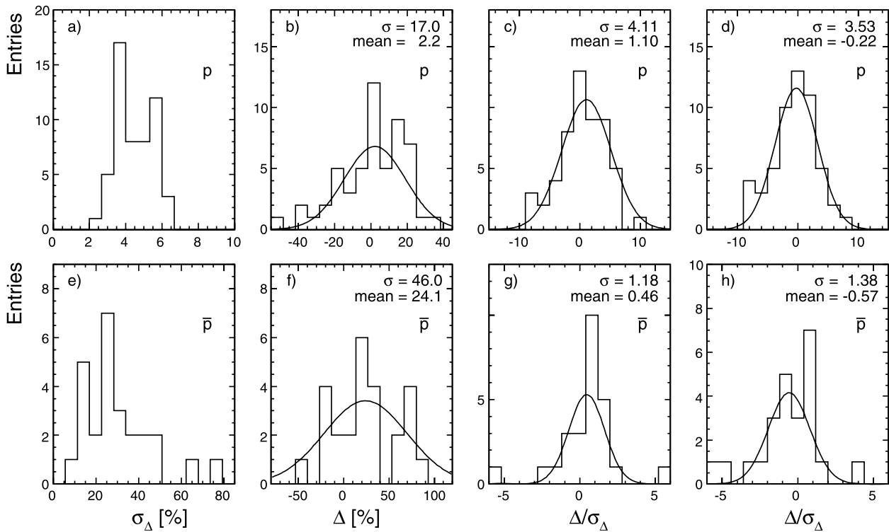
Fig. 35 Statistical analysis of the difference between the measurements of [16] and NA49 for protons ( upper four panels ) and anti-protons ( lower four panels ): ( a ) and ( e ) error of the difference of the
