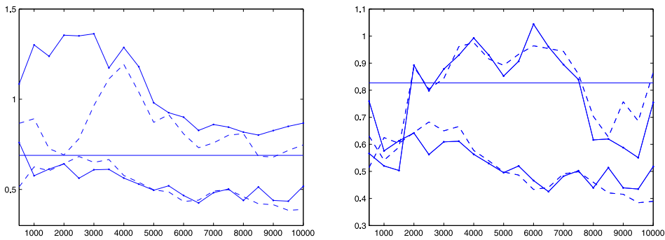
FIG. 3. Estimated 0.95 quantile of the bootstrap distribution while generating the bootstrap samples from \mathbb{F}_n (dashed lines) and \tilde{F}_n (solid-dotted lines) for two independent data sequences along with the 0.95 quantile of the limit distribution of \Delta_n (solid line) for the two models: Exponential(1) (left panel) and |Z| where Z \sim \text{Normal}(0, 1) (right panel).
