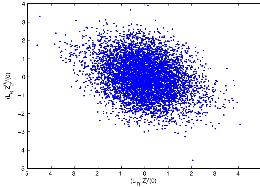
FIG. 1. Scatter plot of 10,000 random draws of ((L_{\mathbb{R}}Z)'(0), (L_{\mathbb{R}}Z_2^0)'(0)) when f(t_0) = 1 and f'(t_0) = -2 .
