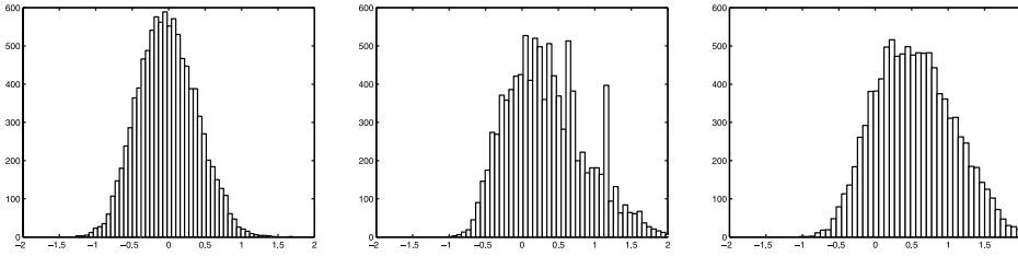
FIG. 2. Histograms of the exact distribution of \Delta_n (left panel) and the two bootstrap distributions while drawing bootstrap samples from \mathbb{F}_n (middle panel) and \tilde{F}_n (right panel) for n = 500 .
