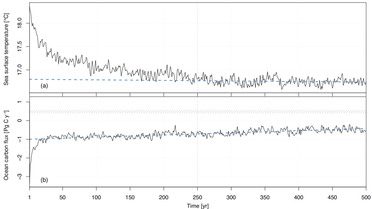
Figure 2. Time series of two climate indices over the 500-year spin-up simulation of IPSL-CM5A-LR. They represent the globally averaged sea surface temperature (a) and the global mean sea-air carbon flux (b). For sea-air carbon flux, negative value indicates uptake of carbon. Steady state equilibrium of physical components as described in Mignot et al. (2013) is reached at \sim 250 years and is indicated with a vertical dashed line. Drifts in sea surface temperature and global carbon flux are indicated with dashed blue lines. They are computed using a linear regression fit over years 250 to 500. Hatching on panel (b) represents the range of inverse modeling estimates for preindustrial global carbon flux as described in Mikaloff Fletcher et al. (2007), i.e., 0.03 \pm 0.08 plus 0.45 \text{ Pg C y}^{-1} corresponding to the riverine-induced natural \text{CO}_2 outgassing outside of near-shore regions consistently with Le Qu  r  t et al. (2015).
