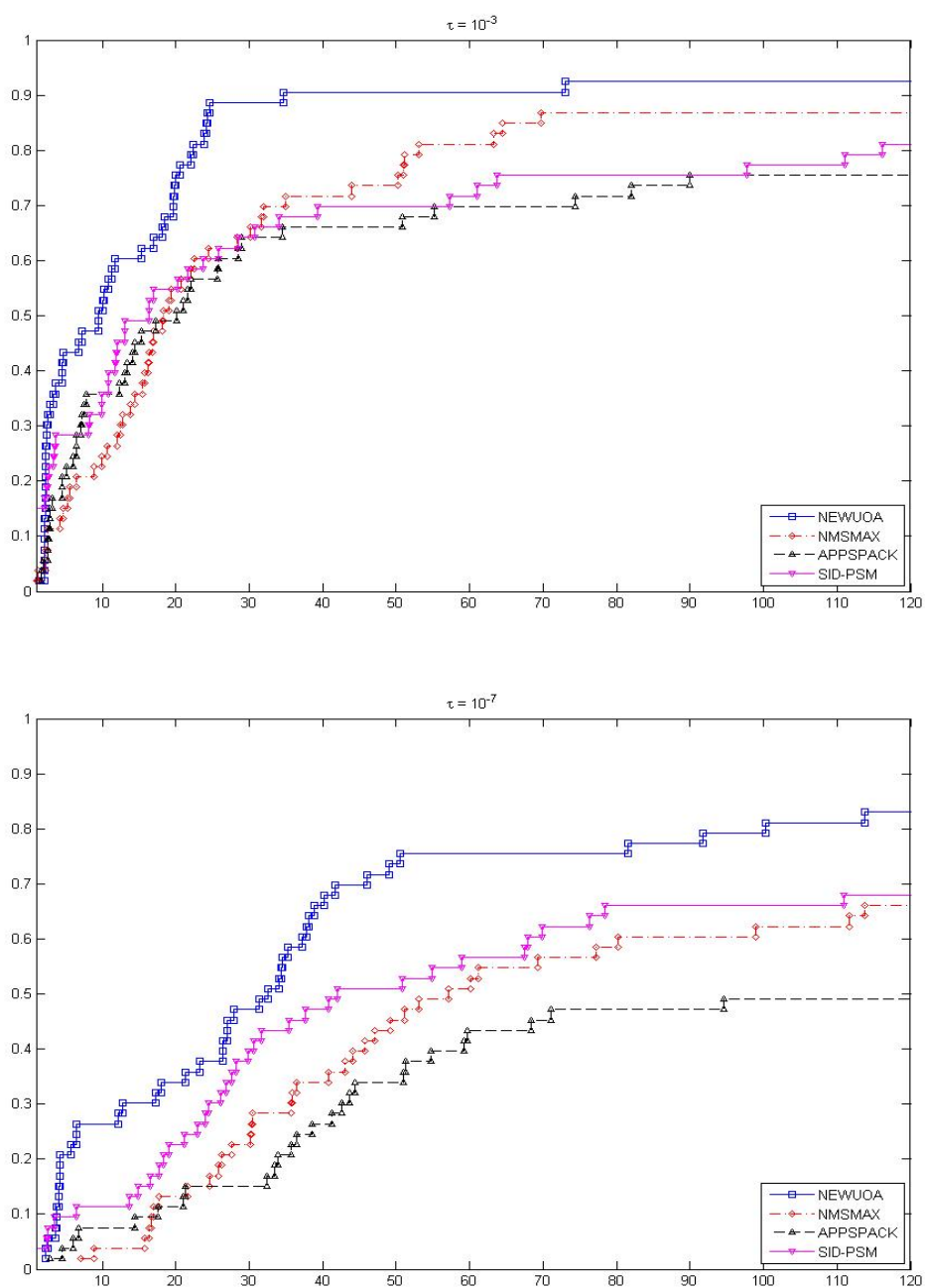
FIGURE 1. Data profiles computed for the set of smooth problems, considering the two levels of accuracy 10^{-3} and 10^{-7} . The profiles are plotted as a function of the budget, expressed in number of simplices of dimension n .
