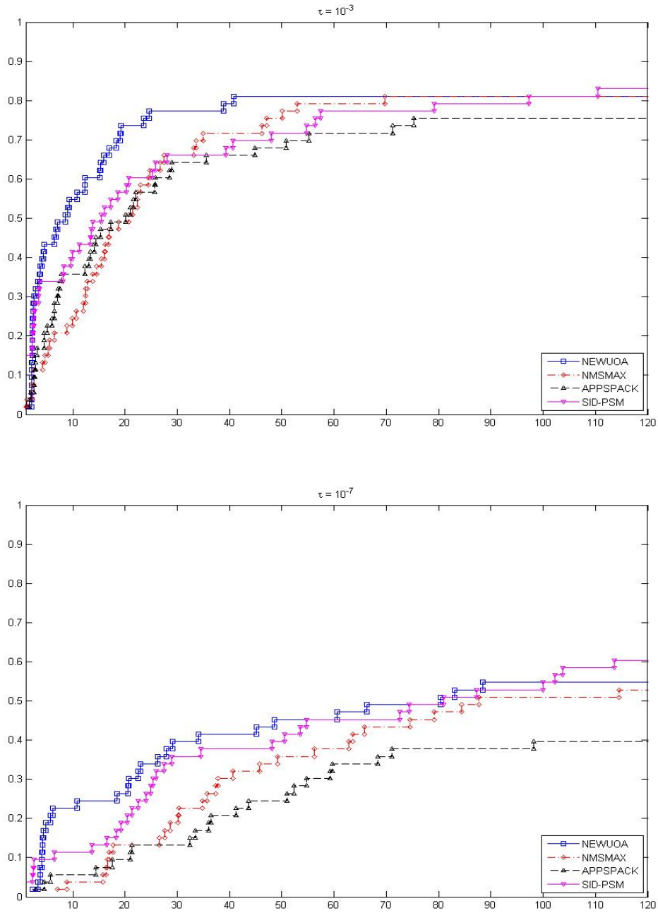
FIGURE 4. Data profiles computed for the set of stochastic noisy problems, considering the two levels of accuracy 10^{-3} and 10^{-7} . The profiles are plotted as a function of the budget, expressed in number of simplices of dimension n .
