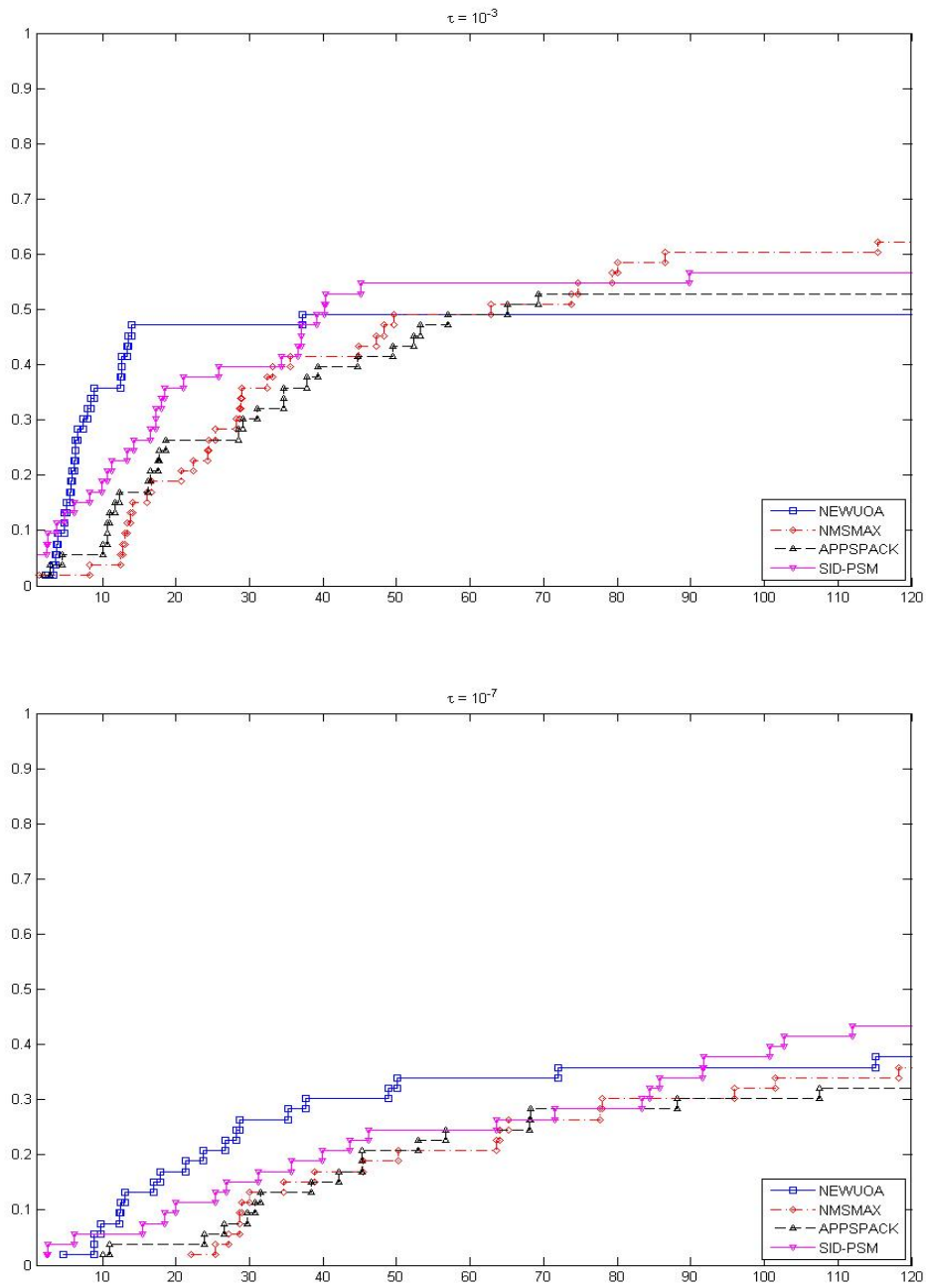
FIGURE 3. Data profiles computed for the set of piecewise smooth problems, considering the two levels of accuracy 10^{-3} and 10^{-7} . The profiles are plotted as a function of the budget, expressed in number of simplices of dimension n .
