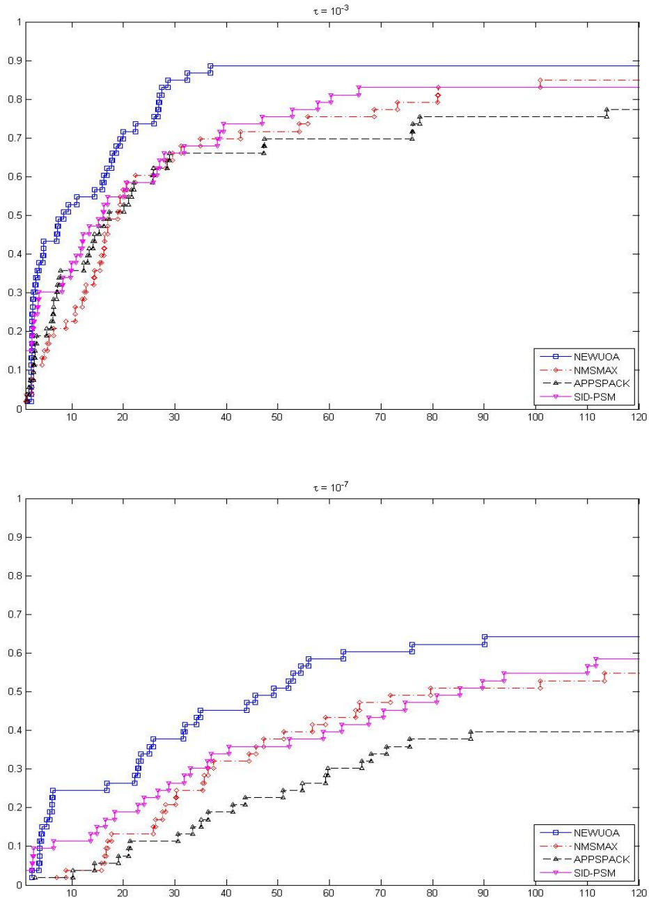
FIGURE 2. Data profiles computed for the set of nonstochastic noisy problems, considering the two levels of accuracy 10^{-3} and 10^{-7} . The profiles are plotted as a function of the budget, expressed in number of simplices of dimension n .
