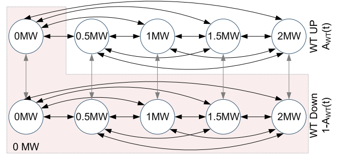
Fig. 7. 2-MW WT availability model—the highlighted states show zero generation due to either wind power unavailability or WT unavailability or both [32], [35], [37].
