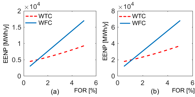
Fig. 16. Impact of WTC and WFC unavailability (FOR) on the EENP by the (a) 40-MW and (b) 160-MW WF.
