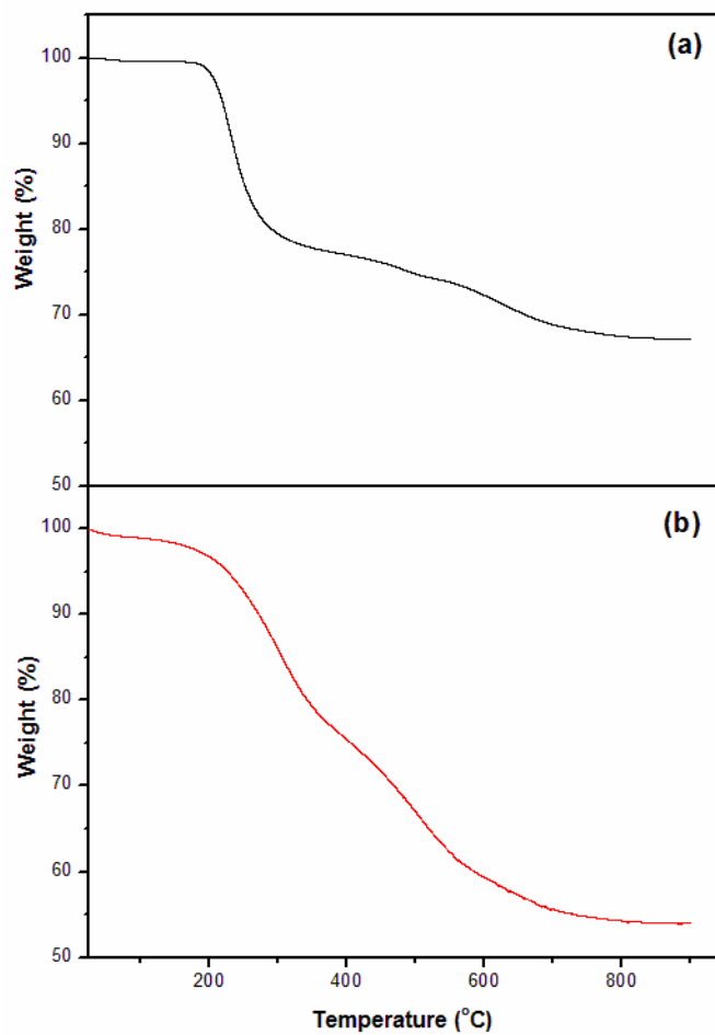
Figure S3. TGA curves of Organo-Sw y-1 (a) and C 60 @Organo-Sw y-1 (b).
