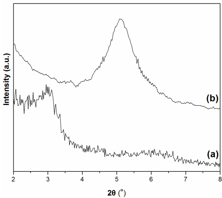
Figure S1. Powder X-Ray diffraction patterns of the starting C_{60}@Organo-SW_{y-1} (a) and the final C_{60}@Al -exchanged- SW_{y-1} (b) samples.
