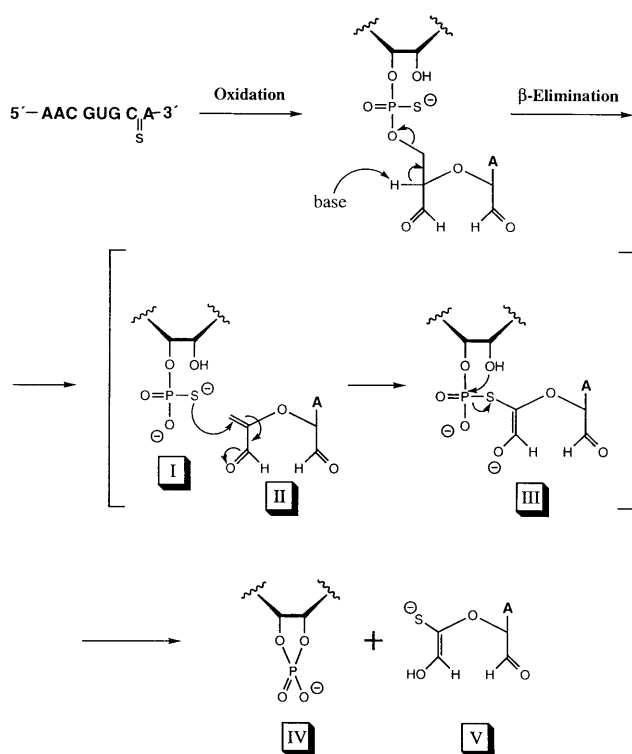
Figure 3. Cleavage of an internucleotidic phosphorothioate in an oligonucleotide.
