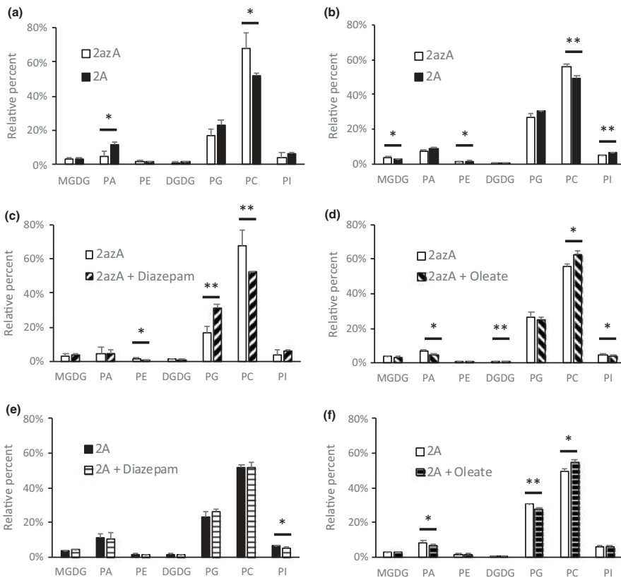
Fig. 5 Relative distribution of ^{14}\text{C} between polar lipid species following incubation of [U-^{14}\text{C}] glycerol with 27 d after flowering (DAF) embryos of lysophosphatidate acyltransferase (LPAAT) overexpressing transgenic line of Brassica napus DH12075 (2A) compared with azygote line (2azA) in the presence or absence of 100 \mu\text{M} diazepam or 1 mM oleate. (a, b) Comparison between uptake of [U-^{14}\text{C}] glycerol into LPAAT overexpressor and azygote line. (c, d) Influence of 100 \mu\text{M} diazepam or 1 mM oleate on an azygote line, respectively. (e, f) Influence of 100 \mu\text{M} diazepam or 1 mM oleate on an LPAT overexpressing line, respectively. Data show means \pm SD ( n = 3 ). (*, P < 0.05 ; **, P < 0.01 , by Student's t -test).
