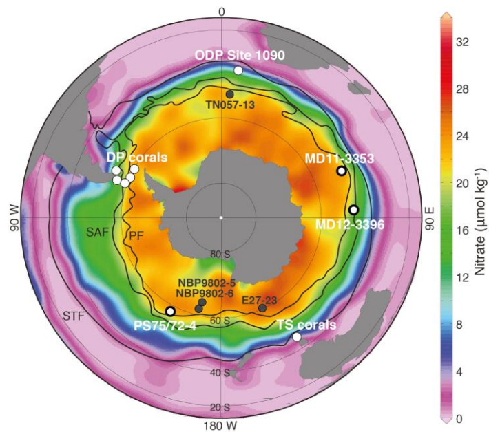
Fig. 1: Sediment core and deep sea coral locations relative to austral summer surface nitrate concentrations and oceanic fronts. Core locations of the diatom-bound \delta^{15}\text{N} and opal flux records are shown in white with a black rim, locations of the ODP Site 1090 foraminifera-bound \delta^{15}\text{N} record and of the coral-bound \delta^{15}\text{N} measurements are shown in white, and sediment cores with published opal flux data mentioned in the text are shown in dark grey. APF, Antarctic Polar Front; SAF, Subantarctic Front; STF, Subtropical Front. Fronts are after Orsi et al. 54 .
