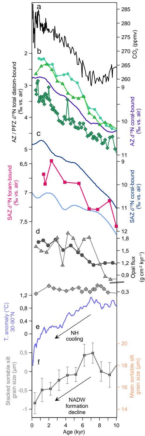
Fig. 2: Holocene records of fossil-bound \delta^{15}\text{N} and biogenic opal flux from the Southern Ocean, compared with climate- and circulation-related records from the Northern Hemisphere and with atmospheric \text{CO}_2 . a, Atmospheric \text{pCO}_2 composite 55 . b, \delta^{15}\text{N} records from the Antarctic Zone of the Southern Ocean. Diatom-bound \delta^{15}\text{N}
