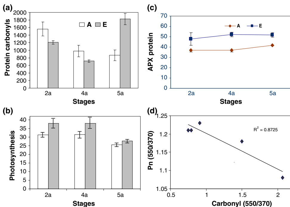
Fig. 5 Effect of elevated [CO 2 ] and stage of plant development on soybean ‘P93B15’ leaf (a) protein carbonylation, (b) leaf photosynthetic rate, and (c) content of APX1 protein, measured by immunoblotting. The most recently fully expanded trifoliolate leaf was harvested at stages 2a (full bloom; day 198), 4a (pod formation; day 213), and 5a (pod fill; day 237). A = ambient [CO 2 ]; E = elevated [CO 2 ]. (d) Inverse relationship between stimulation of Pn at elevated [CO 2 ] and leaf protein carbonyl content, with both parameters expressed as a ratio of values obtained for plants grown at elevated [CO 2 ] (550 ppm) versus ambient [CO 2 ] (370 ppm)
