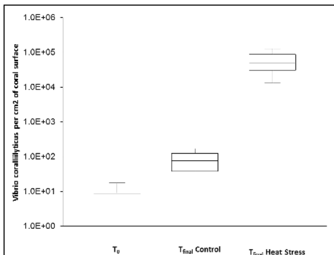
FIGURE 3 | Quantitative PCR assays were used to quantify the abundance of natural populations of Vibrio coralliilyticus associated with the coral P. damicornis on Heron Island, the Great Barrier Reef at t_0 (22°C), t_{\text{final}} Control (22°C), and t_{\text{final}} Heat stress (31°C) conditions, standard curve: R^2 = 0.995 , Eff% = 99.9. Abundances are expressed as the number of bacteria per \text{cm}^2 . n = 3 .
