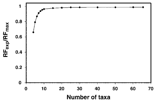
FIGURE 1. Ratio of RF_{exp} to RF_{max} as a function of number of taxa.
