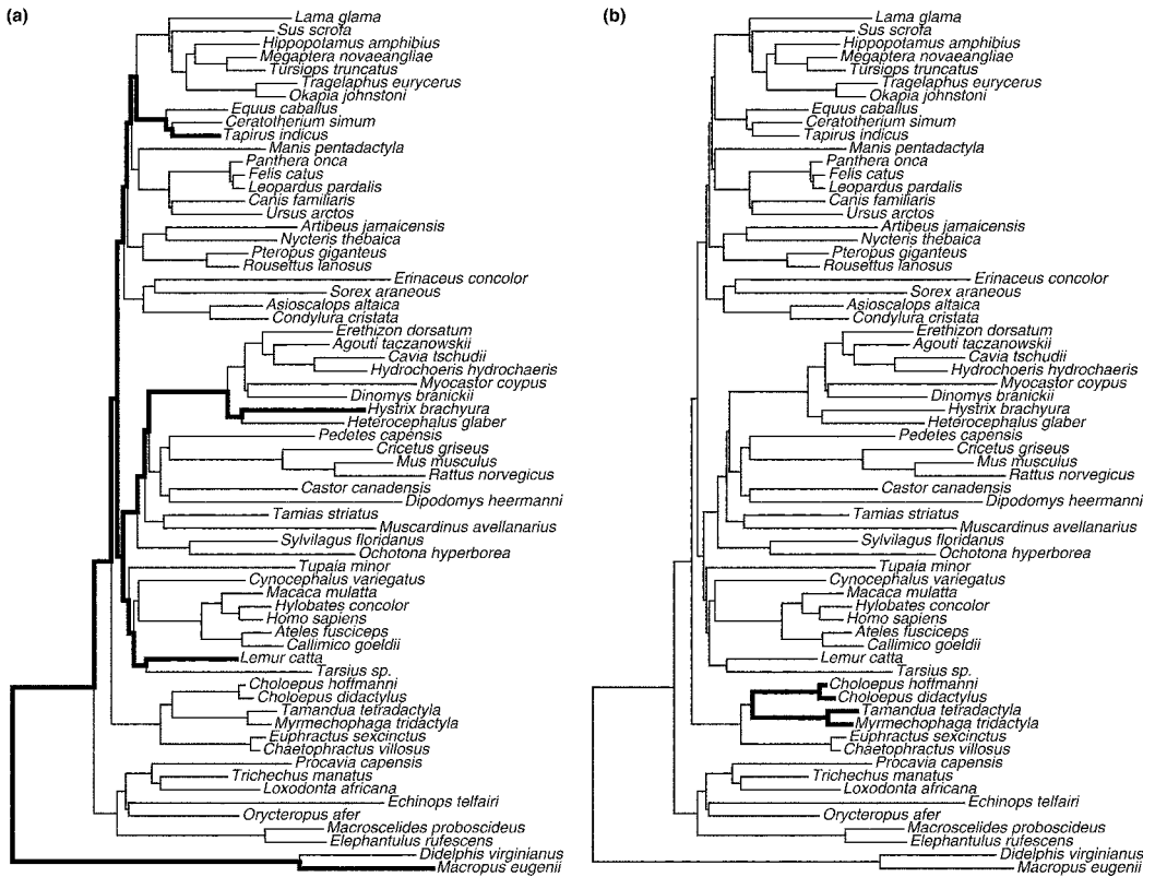
FIGURE 3. Two quartets of taxa sampled from the model tree of Rosenberg and Kumar (2001), shown as heavy lines within the entire model tree. (a) A quartet of large diameter, containing taxa that span the same depth of phylogenetic time as the full data set. (b) A quartet of small diameter, containing taxa that represent complete taxon sampling for a subtree.
