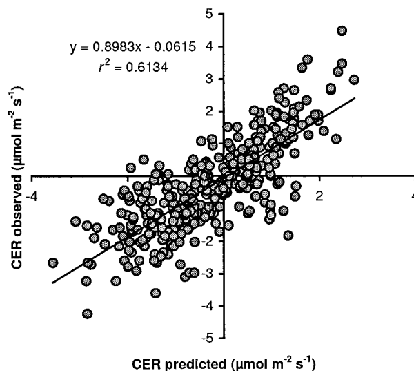
FIGURE 7. Instantaneous observed net ecosystem \text{CO}_2 exchange rate ( \text{CER}_{\text{ecosystem}} ) as a function of instantaneous predicted \text{CER}_{\text{ecosystem}} . Pooled measurements of the whole growing season.
