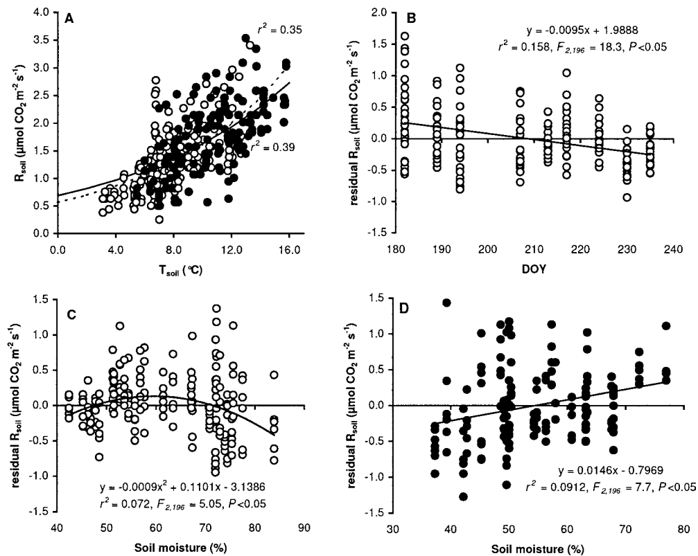
FIGURE 3. (A) Soil respiration ( R_{soil} ), from all measurement days, as a function of soil temperature ( T_{soil} ) at a depth of 2.5 cm. Separate curves are fitted (eq. 3) for control ( \circ , dotted line) and heated ( \bullet , solid line) plots. (B, C) Residual soil respiration (Respiration observed –Respiration fitted ) for control plots as a function of DOY and soil moisture. (D) Residual soil respiration for plots under simulated warming as a function of soil moisture.
