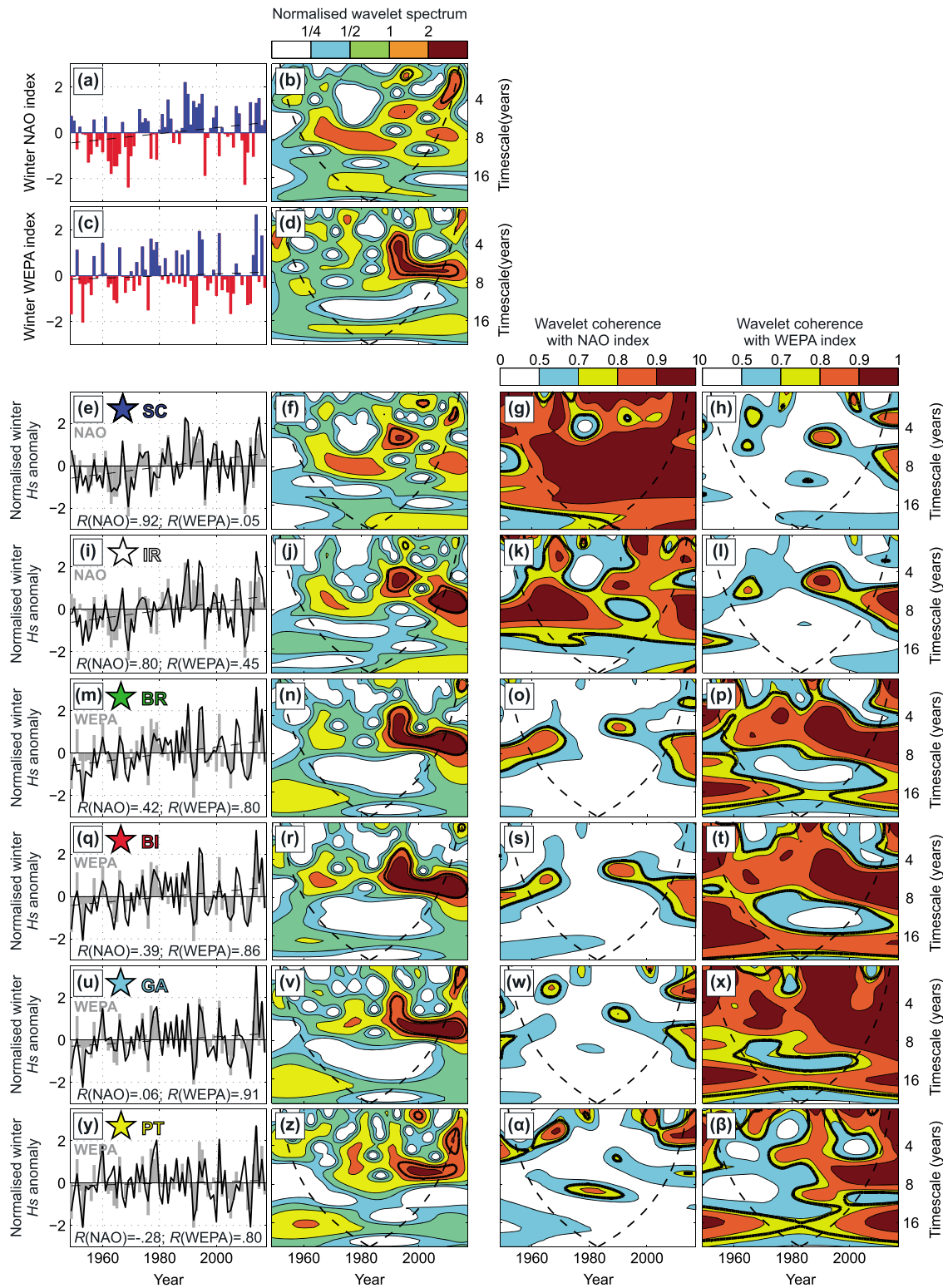
Figure 2. First column: time series of (a) North Atlantic Oscillation (NAO) and (c) West Europe Pressure Anomaly (WEPA) indices, with the six bottom panels showing the time series of the normalized winter-mean H_s anomaly (black line) at the six virtual buoys, and its linear trend (black dotted line) superimposed onto the climate index (gray bars) with which the best correlation is found: (e, i): NAO; (m, q, u, and y): WEPA. Second column: local wavelet spectrum normalized by the variance of the (b) NAO and (d) WEPA indices and (f, j, n, r, v, and z) of the normalized winter H_s anomaly at the six virtual buoys. Third and fourth columns show the wavelet coherency-squared diagram normalized with the variance between the winter H_s at the six virtual buoys and the (g, k, o, s, w, and \alpha ) NAO and (h, l, p, t, x, and \beta ) WEPA indices, respectively. In all wavelet panels, the 5% significance level against red noise is contoured in black thick line and the cone of influence is delimited by the black dashed line.
