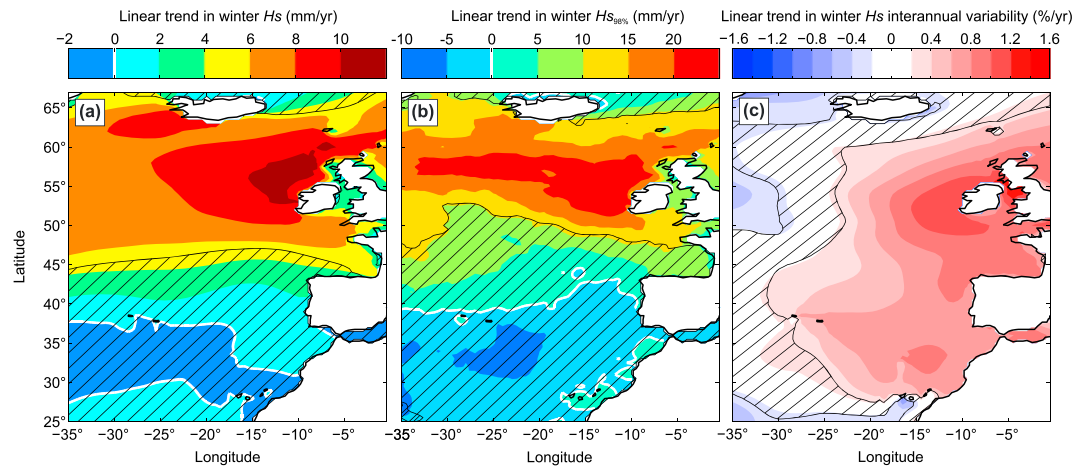
Figure 3. Linear trend of (a) winter-mean (1949–2017) H_s and (b) its 98% exceedance values H_{s_{98\%}} in millimeter/year and of (c) winter-mean (1949–2017) H_s interannual variability in percent/year. The hatched zones are areas where trends and correlations are not significant at the 95% confidence level.
