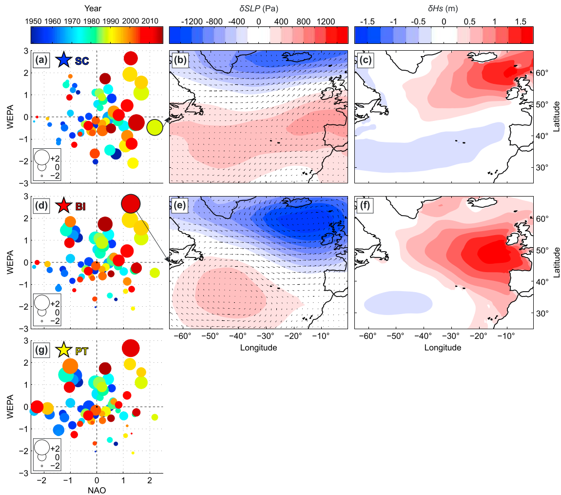
Figure 4. First column: West Europe Pressure Anomaly (WEPA) index versus North Atlantic Oscillation (NAO) index for the 69 December to March winters (1949–2017) with the winter year colored and the circle size proportional to the normalized winter-mean H_s anomaly at the buoys (a) SC: Scotland, (d) BI: Biscay, and (g) PT: Portugal. Second and third columns: The atmospheric and wave height expression of the two winters with (b, c) the highest Hurrell-definition NAO index (1988/1989) and (e, f) the highest WEPA index (2013/2014) with (b, e) the winter-mean sea level pressure (SLP) anomaly with superimposed \bar{u}_{10} field and (c, f) the winter-mean H_s anomaly.
