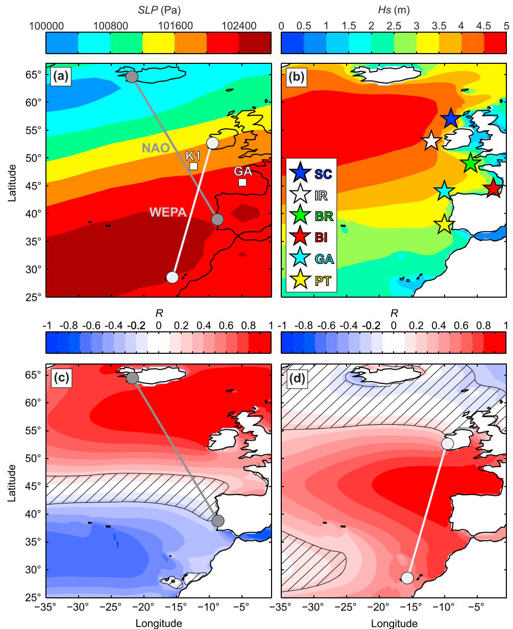
Figure 1. Top panels: winter-mean (December to March, 1949–2017). (a) sea level pressure (SLP) and (b) H_s . Bottom panels: spatial correlation of the winter-mean H_s against the (December to March) winter-averaged (c) NAO and (d) WEPA indices. The North Atlantic Oscillation (NAO) and West Europe Pressure Anomaly (WEPA) indices defined as the normalized SLP difference measured between two stations are indicated by the dark and light gray circles in panels (a, c, and d). The two white squares in (a) K1 and GA indicate the location of two relevant operated wave buoys used for validation. The six virtual wave buoys along the west coast of Europe are shown in panel (b), with SC = Scotland; IR = Ireland; BR = Brittany; BI = Biscay; GA = Galicia; PT = Portugal. The hatched zones are the areas where correlations are not significant at the 95% confidence level.
