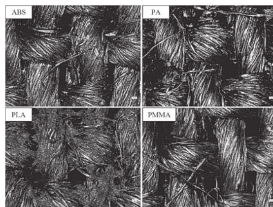
Figure 1: CLSM images of polymer-coated samples (nominal magnification 400 \times )
