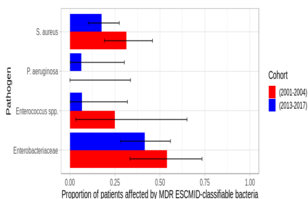
Figure 1: Comparison of microbiology between patients treated in 2001-2004 and 2013-2017 depicting the change in the proportion of patients affected by multi-drug resistant (MDR) ESCMID-classifiable bacteria. This demonstrates the reduction in both resistant Staphylococci (including MRSA) and resistant Enterobacteriaceae isolated over the 10-year period as described in the text. In addition, the reduction in the proportion of patients affected by MDR Enterococcus species isolated from patients managed at our institution over the same time period is shown. Adapted from Dudareva et al et al. 3
