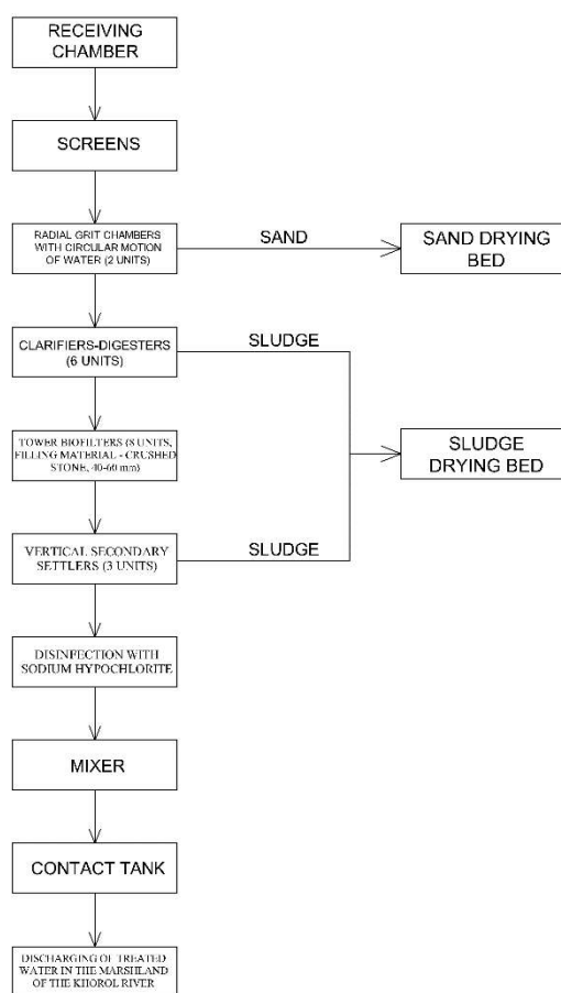
Fig. 1. Wastewater treatment process scheme at Khorol factory for baby food
