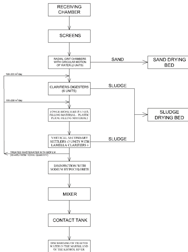
Fig. 4. Improved wastewater treatment process scheme of Khorol factory for baby food
