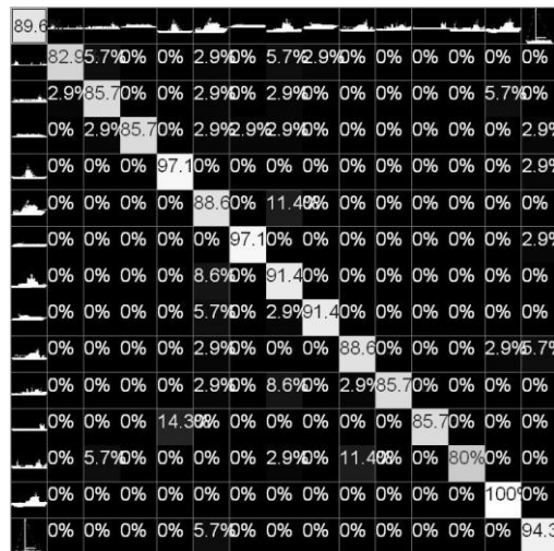
Figure 3 Vessel Classification Algorithm Performance
