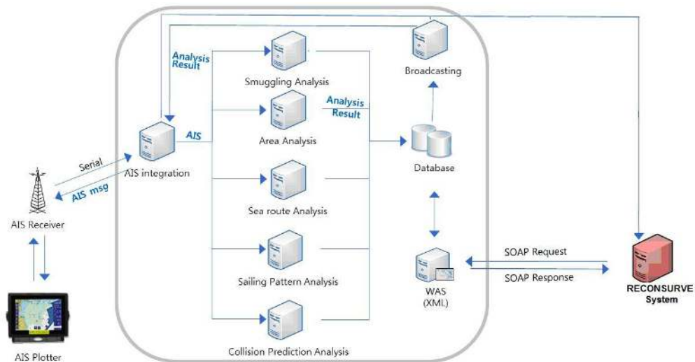
Figure 2 AIS Data Gathering and Integration
