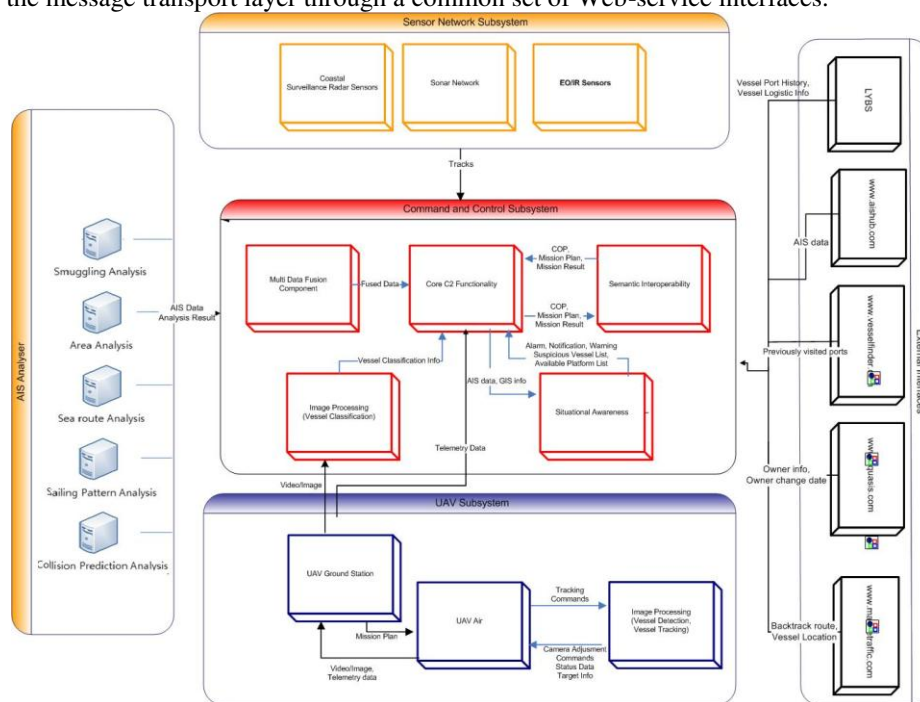
Figure 4 Interoperating Data Sources: Data Flow
