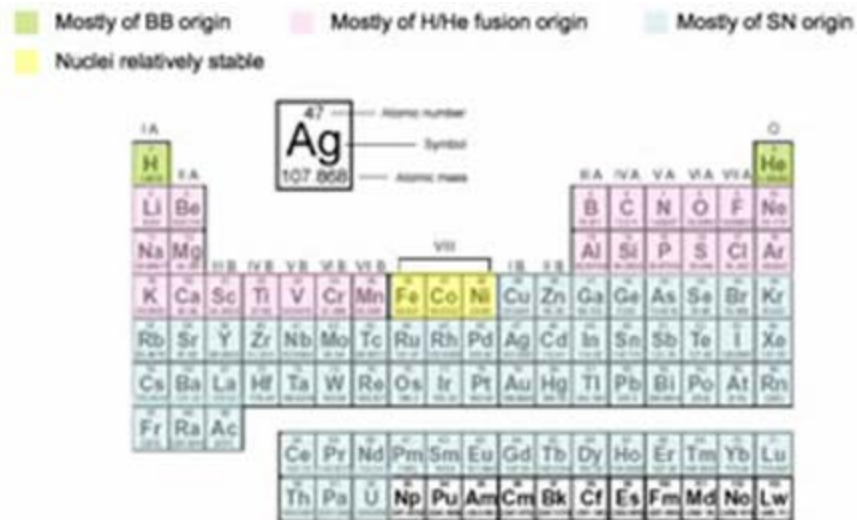
Figure 5. Periodic table presented by Rick Lee from General Atomic Fusion Lab.
