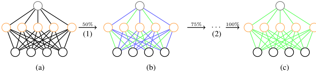
Figure 1: An overview of our incremental network quantization method. (a) Pre-trained full-precision model used as a reference. (b) Model update with three proposed operations: weight partition, group-wise quantization (green connections) and re-training (blue connections). (c) Final low-precision model with all the weights constrained to be either powers of two or zero. In the figure, operation (1) represents a single run of (b), and operation (2) denotes the procedure of repeating operation (1) on the latest re-trained weight group until all the non-zero weights are quantized. Our method does not lead to accuracy loss when using 5-bit, 4-bit and even 3-bit approximations in network quantization. For better visualization, here we just use a 3-layer fully connected network as an illustrative example, and the newly re-trained weights are divided into two disjoint groups of the same size at each run of operation (1) except the last run which only performs quantization on the re-trained floating-point weights occupying 12.5% of the model weights.
