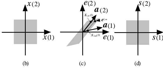
Figure 1. Mixture and separation of independent signals; (a) flow of the signals, (b) an example of probability density distribution of x_{l,m}(1) and x_{l,m}(2) , (c) e_{l,m}(1) and e_{l,m}(2) , and (d) s_{l,m}(1) and s_{l,m}(2) .
