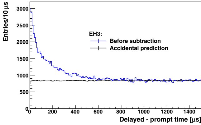
FIG. 3 (color online). Distribution of the delayed minus prompt time of the EH3 data sample. The blue histogram shows coincidences after all cuts except on the time difference. The black curve shows the predicted distribution for accidental coincidences.
