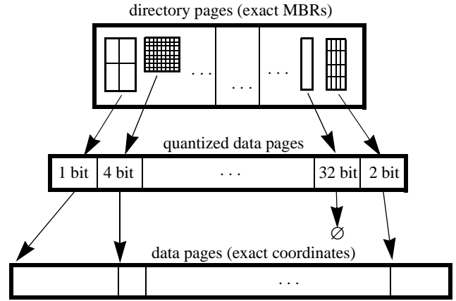
Figure 3: Structure of the IQ-tree
