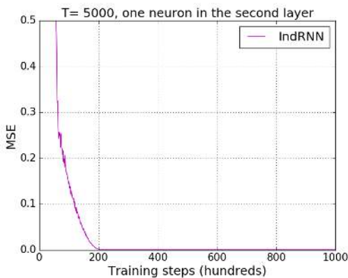
Figure 4. Result of the adding problem with just one neuron in the second layer for sequences of length 5000.
